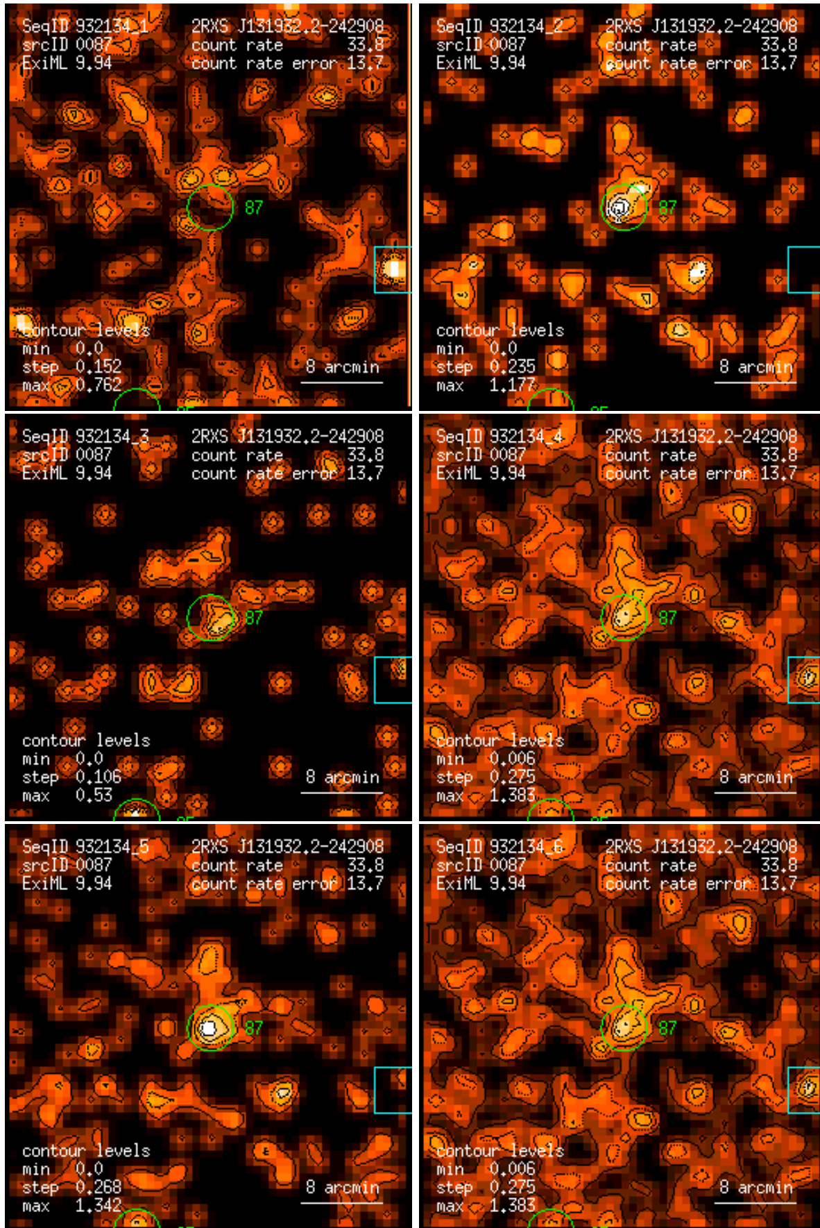
Figure 87: RASS 932134: detection 0087: band rate images, Gaussian filter: (1) PSPC channels 11 – 41, (2) 52 – 90, (3) 91 – 201, (4) 11 – 235, (5) 52 – 201, (6) 11 – 201. Broad band rates in counts/ks. Band rate contour levels in counts/ks/arcmin 2 .
