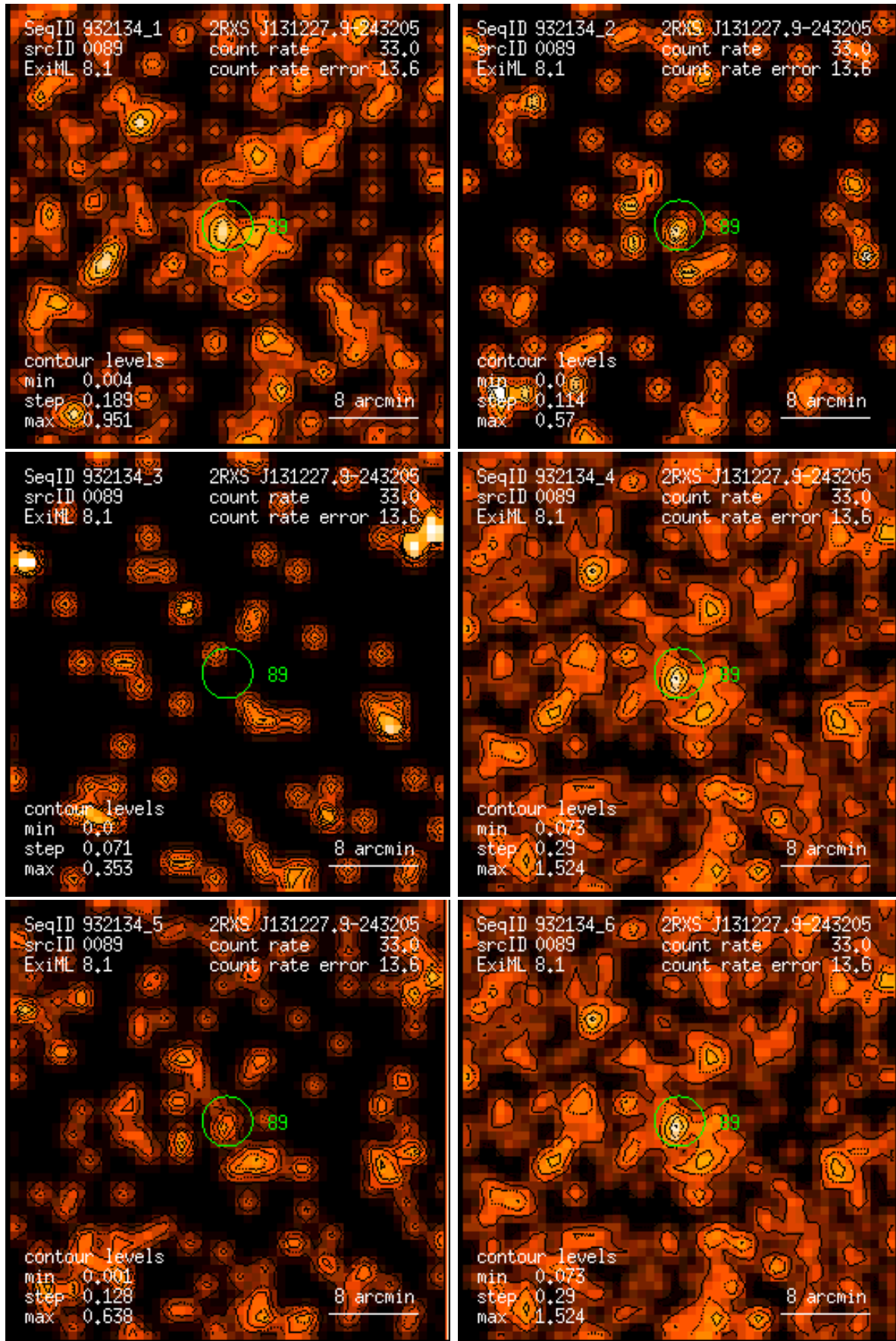
Figure 89: RASS 932134: detection 0089: band rate images, Gaussian filter: (1) PSPC channels 11 – 41, (2) 52 – 90, (3) 91 – 201, (4) 11 – 235, (5) 52 – 201, (6) 11 – 201. Broad band rates in counts/ks. Band rate contour levels in counts/ks/arcmin 2 .
