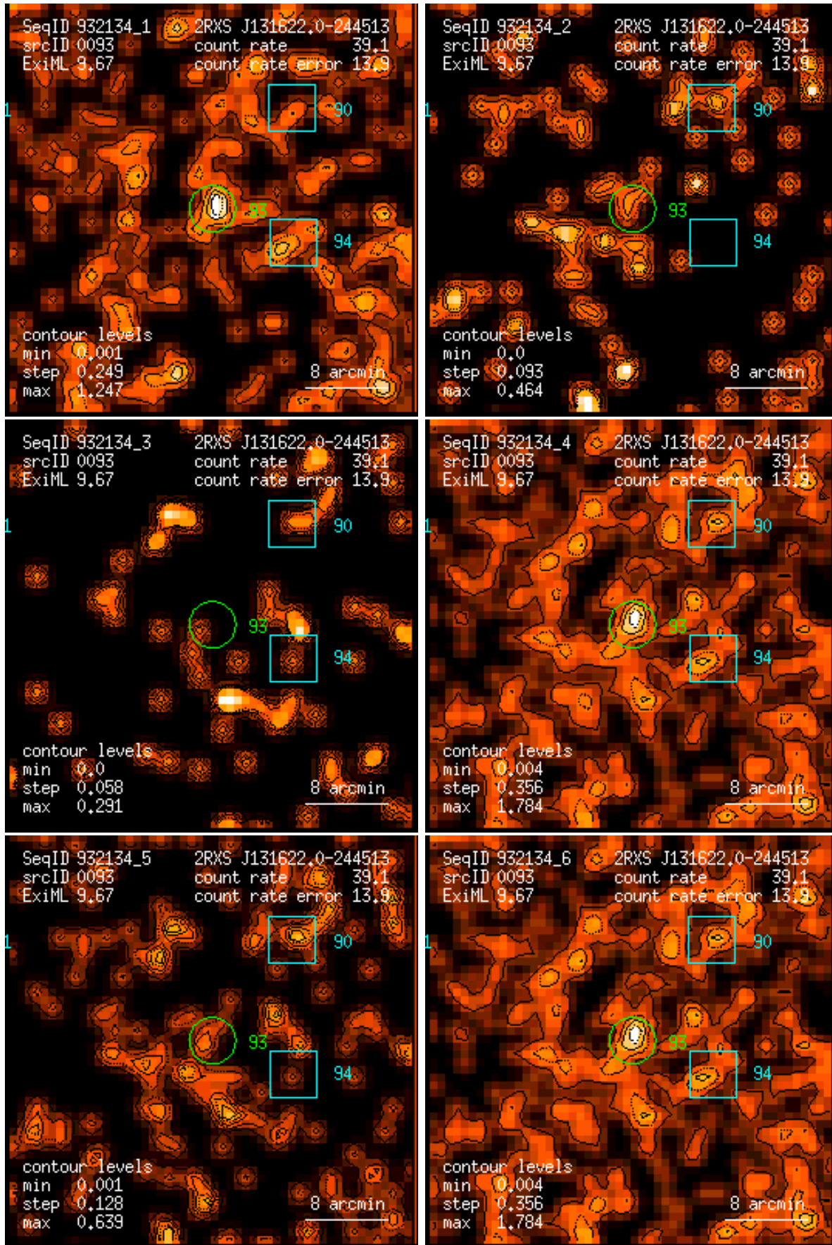
Figure 93: RASS 932134: detection 0093: band rate images, Gaussian filter: (1) PSPC channels 11 – 41, (2) 52 – 90, (3) 91 – 201, (4) 11 – 235, (5) 52 – 201, (6) 11 – 201. Broad band rates in counts/ks. Band rate contour levels in counts/ks/arcmin 2 .
