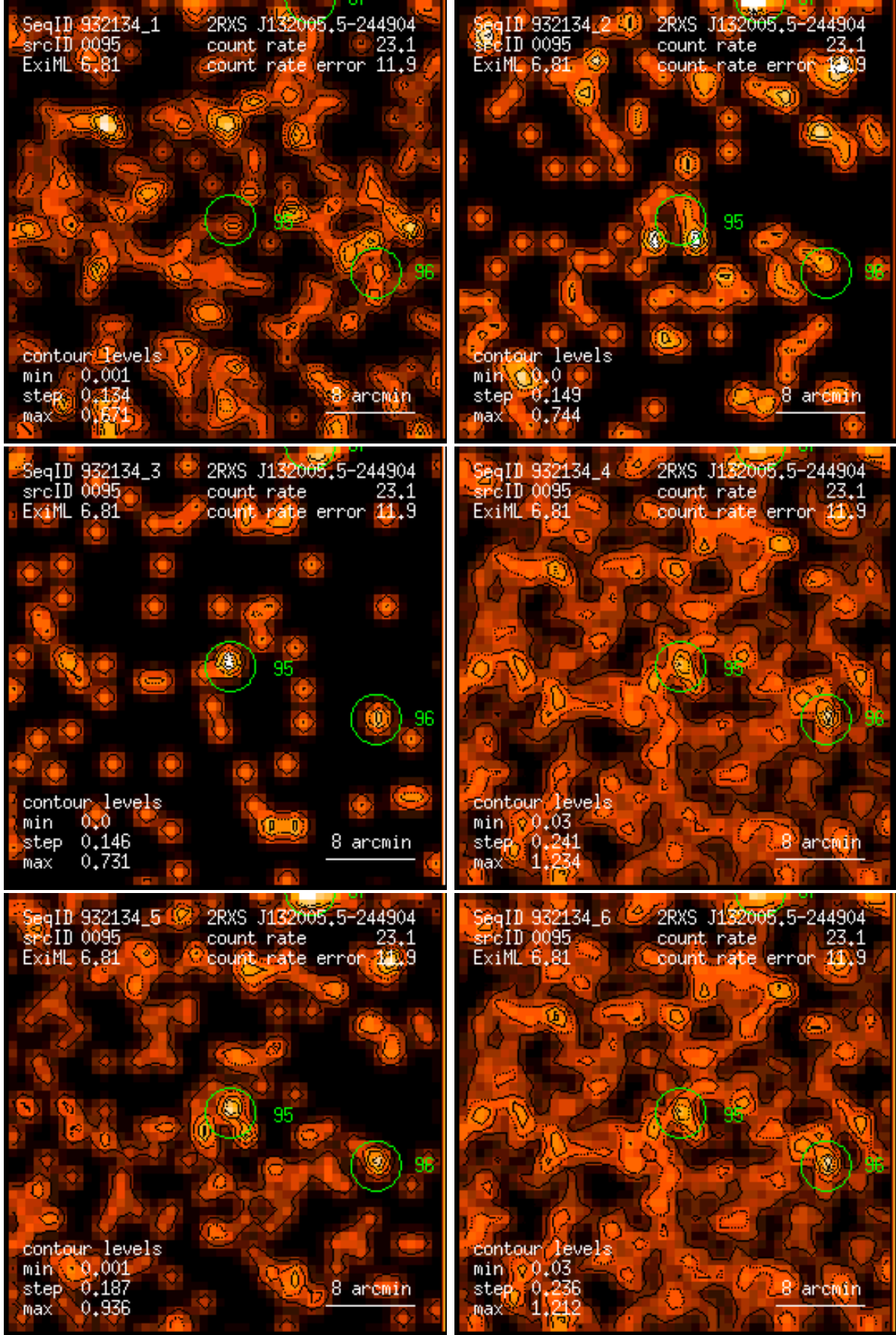
Figure 95: RASS 932134: detection 0095: band rate images, Gaussian filter: (1) PSPC channels 11 – 41, (2) 52 – 90, (3) 91 – 201, (4) 11 – 235, (5) 52 – 201, (6) 11 – 201. Broad band rates in counts/ks. Band rate contour levels in counts/ks/arcmin 2 .
