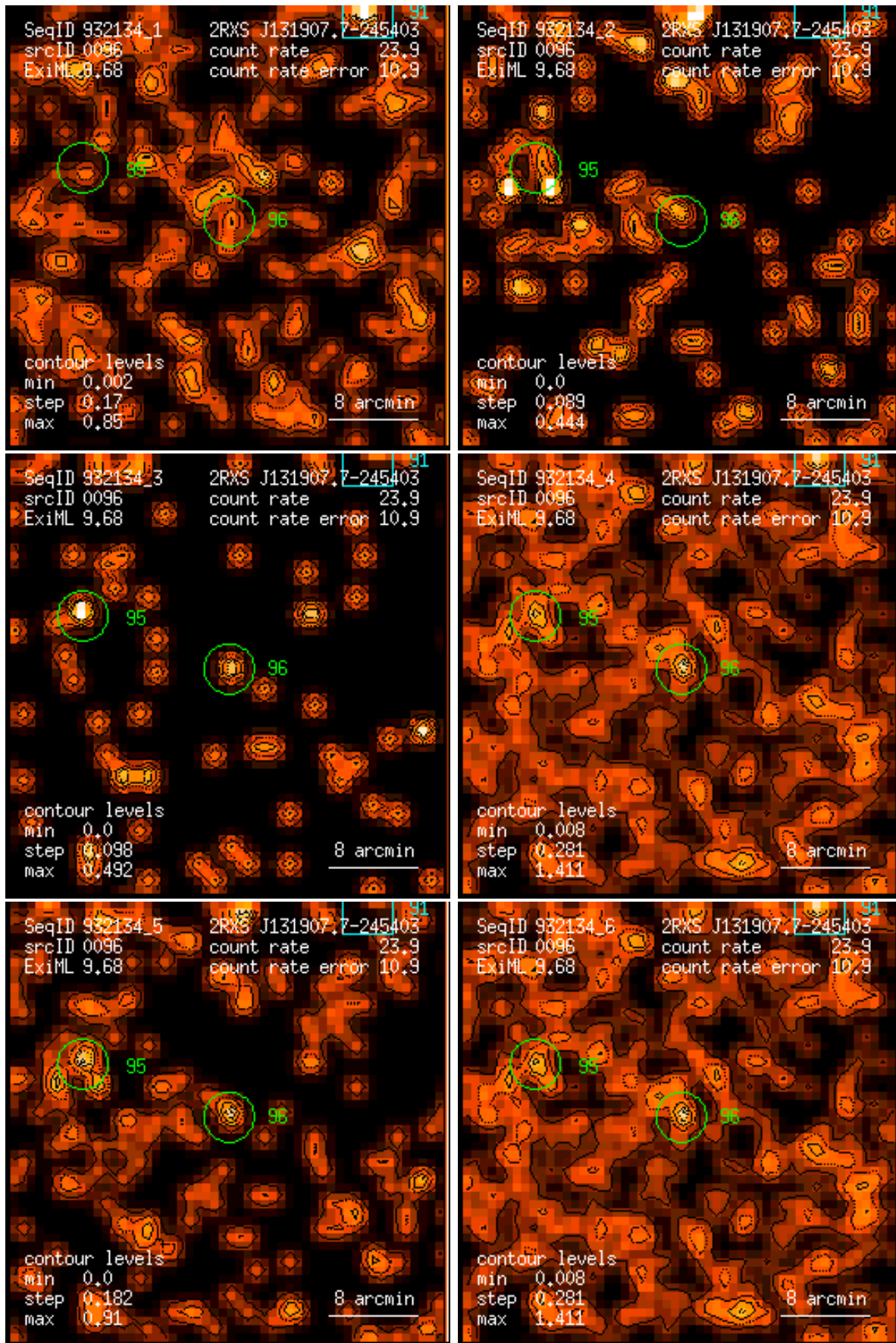
Figure 96: RASS 932134: detection 0096: band rate images, Gaussian filter: (1) PSPC channels 11 – 41, (2) 52 – 90, (3) 91 – 201, (4) 11 – 235, (5) 52 – 201, (6) 11 – 201. Broad band rates in counts/ks. Band rate contour levels in counts/ks/arcmin 2 .
