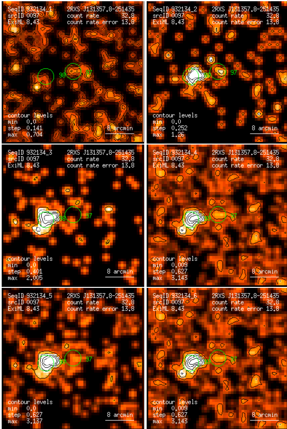
Figure 97: RASS 932134: detection 0097: band rate images, Gaussian filter: (1) PSPC channels 11 – 41, (2) 52 – 90, (3) 91 – 201, (4) 11 – 235, (5) 52 – 201, (6) 11 – 201. Broad band rates in counts/ks. Band rate contour levels in counts/ks/arcmin 2 .
