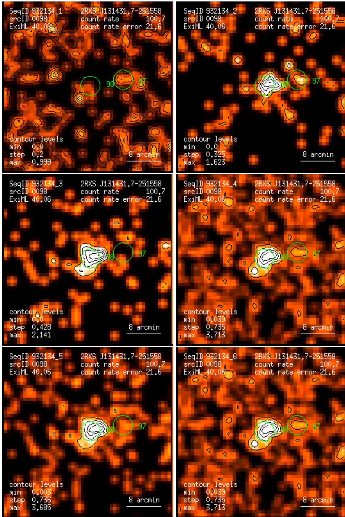
Figure 98: RASS 932134: detection 0098: band rate images, Gaussian filter: (1) PSPC channels 11 – 41, (2) 52 – 90, (3) 91 – 201, (4) 11 – 235, (5) 52 – 201, (6) 11 – 201. Broad band rates in counts/ks. Band rate contour levels in counts/ks/arcmin 2 .
