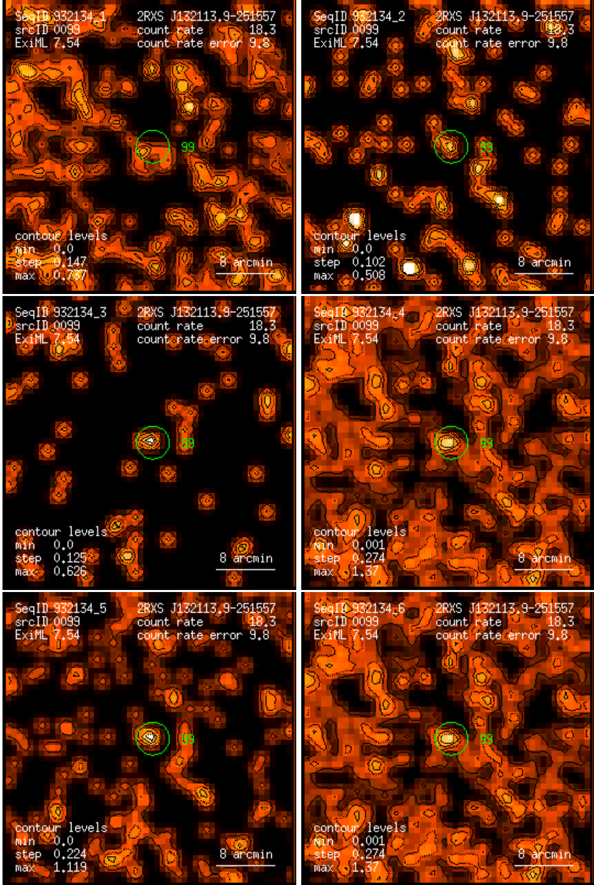
Figure 99: RASS 932134: detection 0099: band rate images, Gaussian filter: (1) PSPC channels 11 – 41, (2) 52 – 90, (3) 91 – 201, (4) 11 – 235, (5) 52 – 201, (6) 11 – 201. Broad band rates in counts/ks. Band rate contour levels in counts/ks/arcmin 2 .
