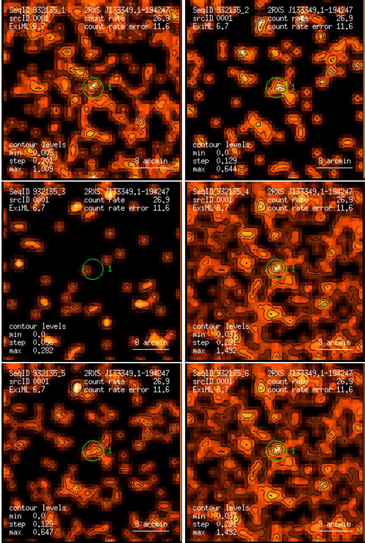
Figure 1: RASS 932135: detection 0001: band rate images, Gaussian filter: (1) PSPC channels 11 – 41, (2) 52 – 90, (3) 91 – 201, (4) 11 – 235, (5) 52 – 201, (6) 11 – 201. Broad band rates in counts/ks. Band rate contour levels in counts/ks/arcmin 2 .
