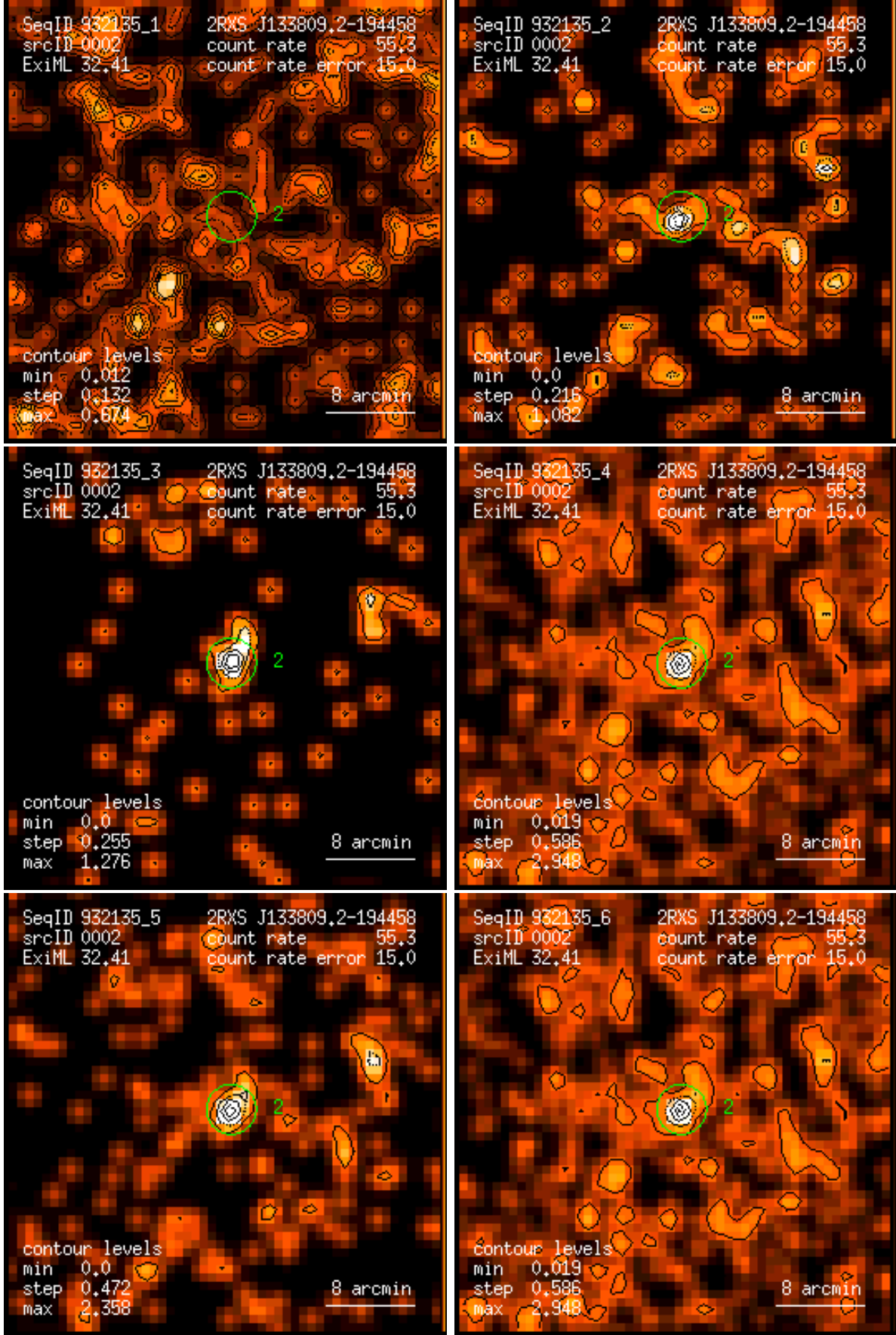
Figure 2: RASS 932135: detection 0002: band rate images, Gaussian filter: (1) PSPC channels 11 – 41, (2) 52 – 90, (3) 91 – 201, (4) 11 – 235, (5) 52 – 201, (6) 11 – 201. Broad band rates in counts/ks. Band rate contour levels in counts/ks/arcmin 2 .
