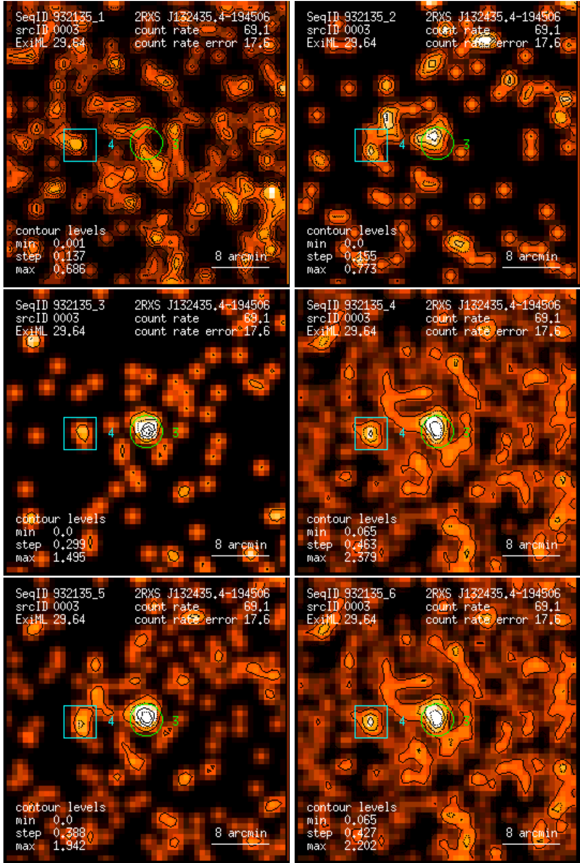
Figure 3: RASS 932135: detection 0003: band rate images, Gaussian filter: (1) PSPC channels 11 – 41, (2) 52 – 90, (3) 91 – 201, (4) 11 – 235, (5) 52 – 201, (6) 11 – 201. Broad band rates in counts/ks. Band rate contour levels in counts/ks/arcmin 2 .
