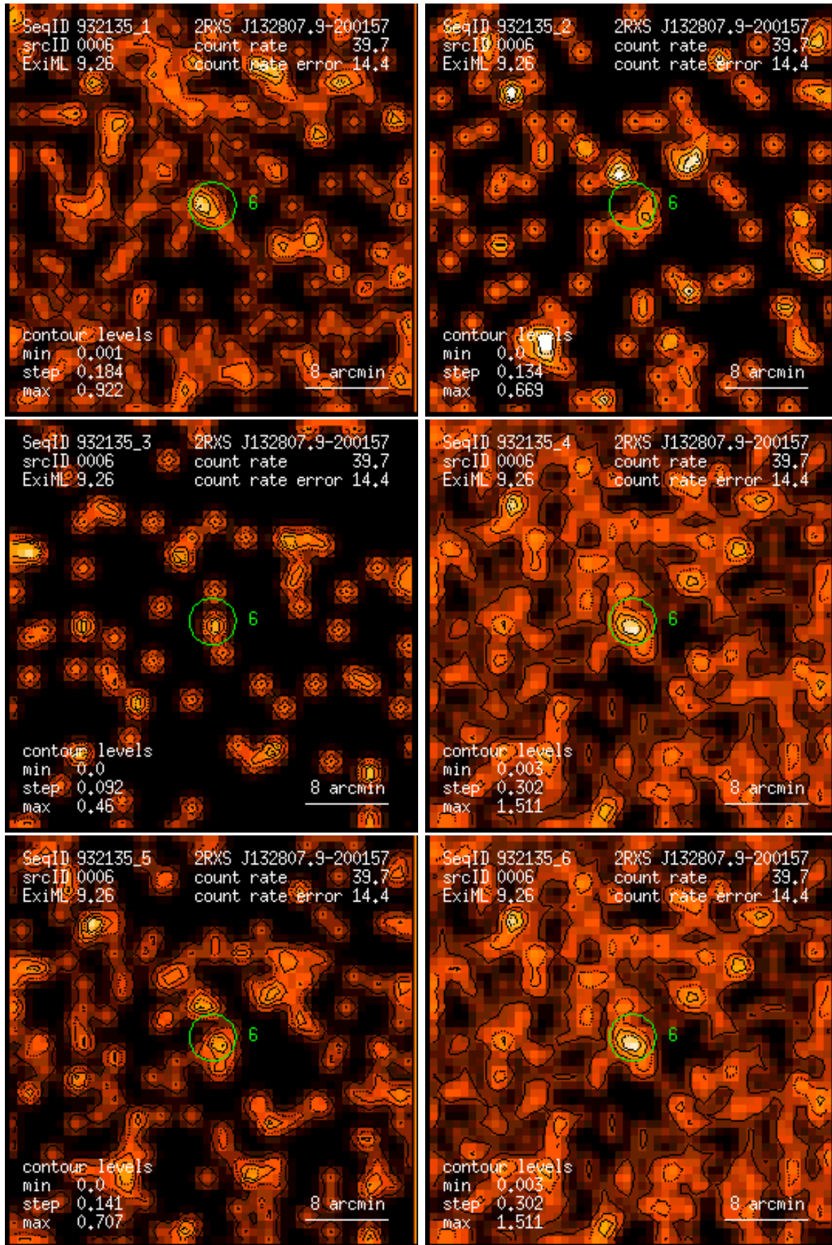
Figure 6: RASS 932135: detection 0006: band rate images, Gaussian filter: (1) PSPC channels 11 – 41, (2) 52 – 90, (3) 91 – 201, (4) 11 – 235, (5) 52 – 201, (6) 11 – 201. Broad band rates in counts/ks. Band rate contour levels in counts/ks/arcmin 2 .
