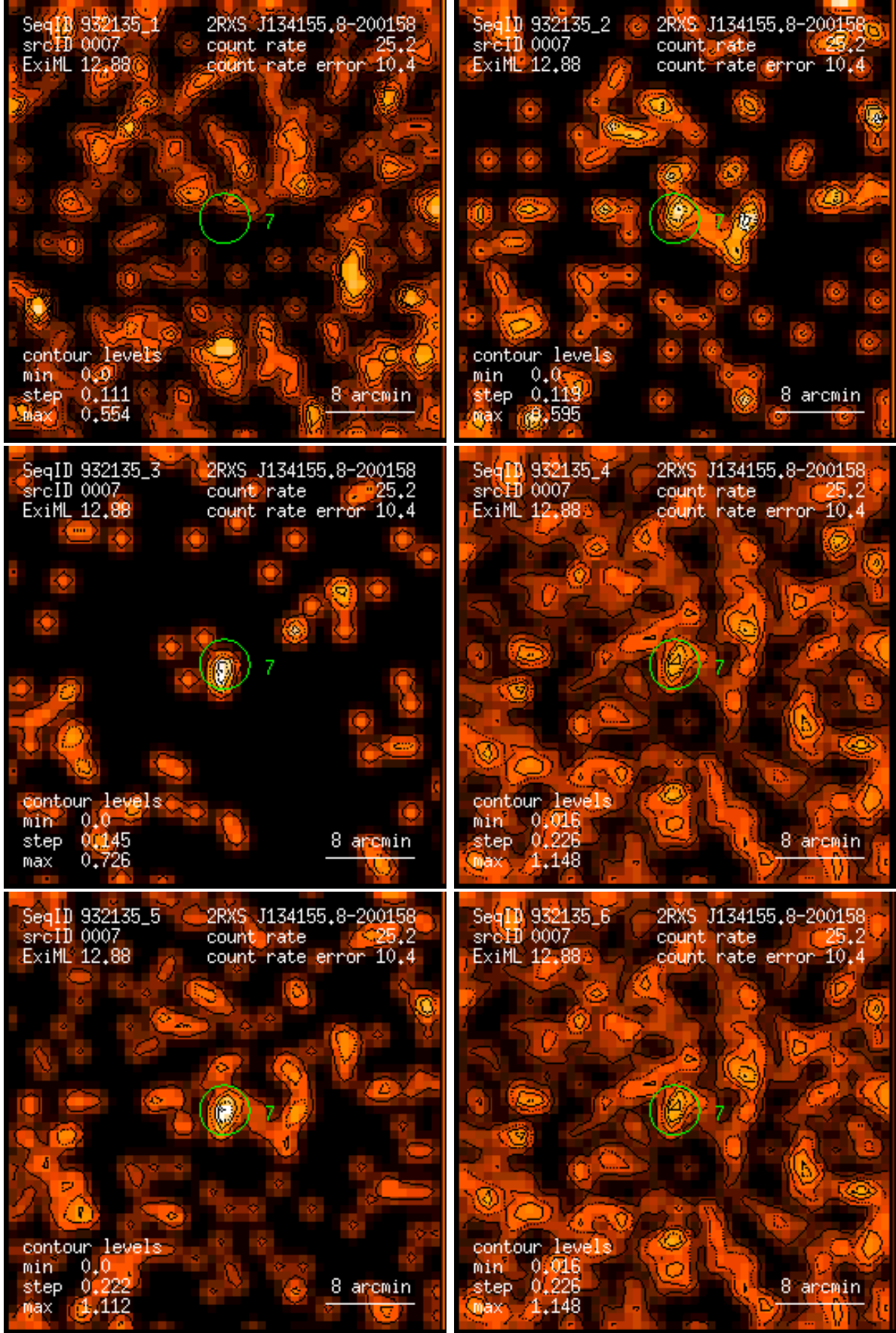
Figure 7: RASS 932135: detection 0007: band rate images, Gaussian filter: (1) PSPC channels 11 – 41, (2) 52 – 90, (3) 91 – 201, (4) 11 – 235, (5) 52 – 201, (6) 11 – 201. Broad band rates in counts/ks. Band rate contour levels in counts/ks/arcmin 2 .
