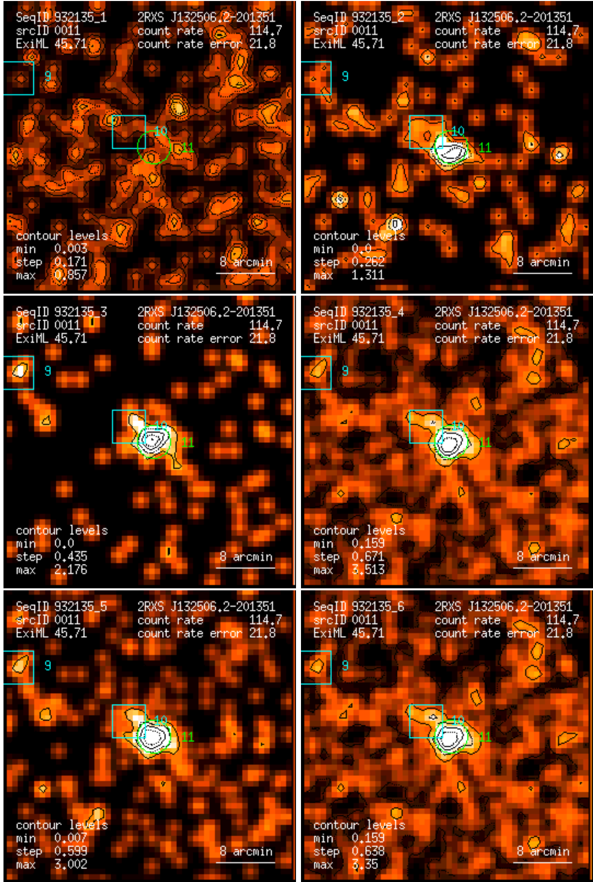
Figure 11: RASS 932135: detection 0011: band rate images, Gaussian filter: (1) PSPC channels 11 – 41, (2) 52 – 90, (3) 91 – 201, (4) 11 – 235, (5) 52 – 201, (6) 11 – 201. Broad band rates in counts/ks. Band rate contour levels in counts/ks/arcmin 2 .
