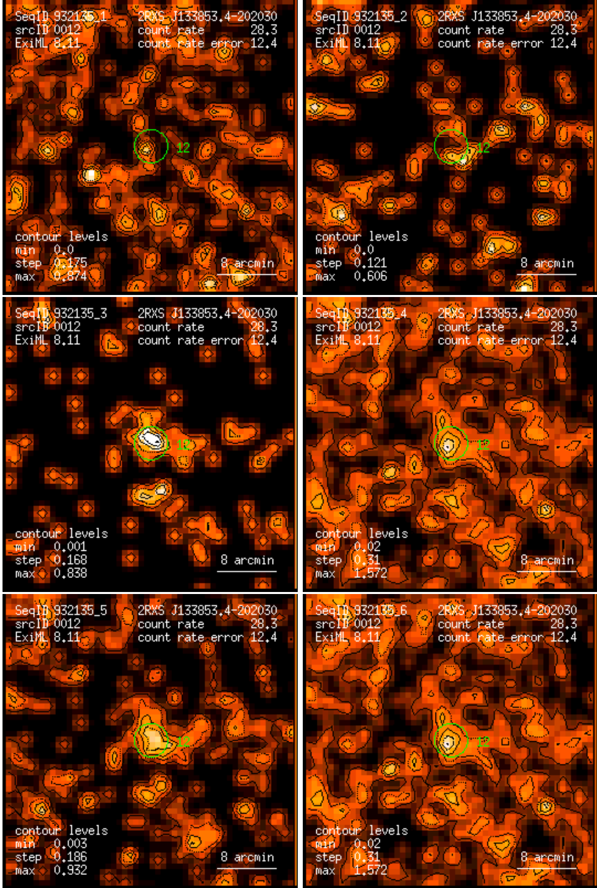
Figure 12: RASS 932135: detection 0012: band rate images, Gaussian filter: (1) PSPC channels 11 – 41, (2) 52 – 90, (3) 91 – 201, (4) 11 – 235, (5) 52 – 201, (6) 11 – 201. Broad band rates in counts/ks. Band rate contour levels in counts/ks/arcmin 2 .
