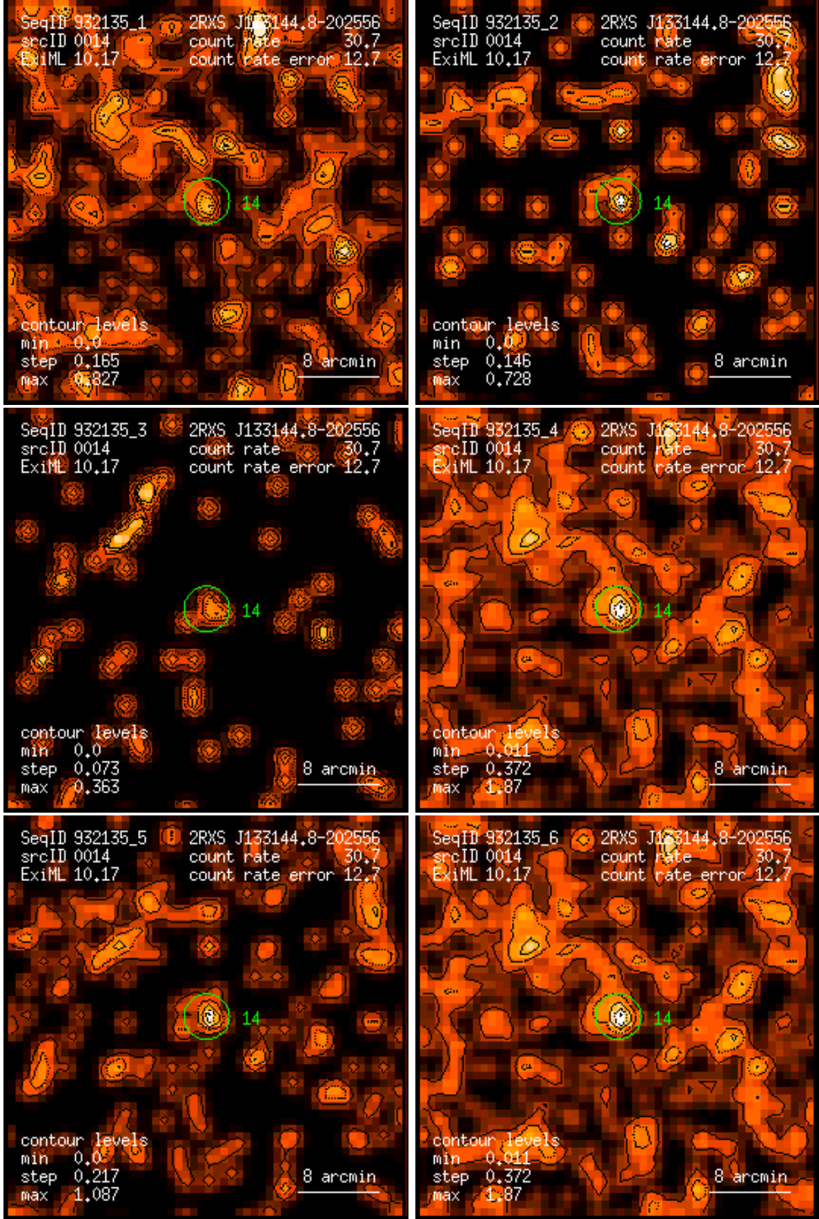
Figure 14: RASS 932135: detection 0014: band rate images, Gaussian filter: (1) PSPC channels 11 – 41, (2) 52 – 90, (3) 91 – 201, (4) 11 – 235, (5) 52 – 201, (6) 11 – 201. Broad band rates in counts/ks. Band rate contour levels in counts/ks/arcmin 2 .
