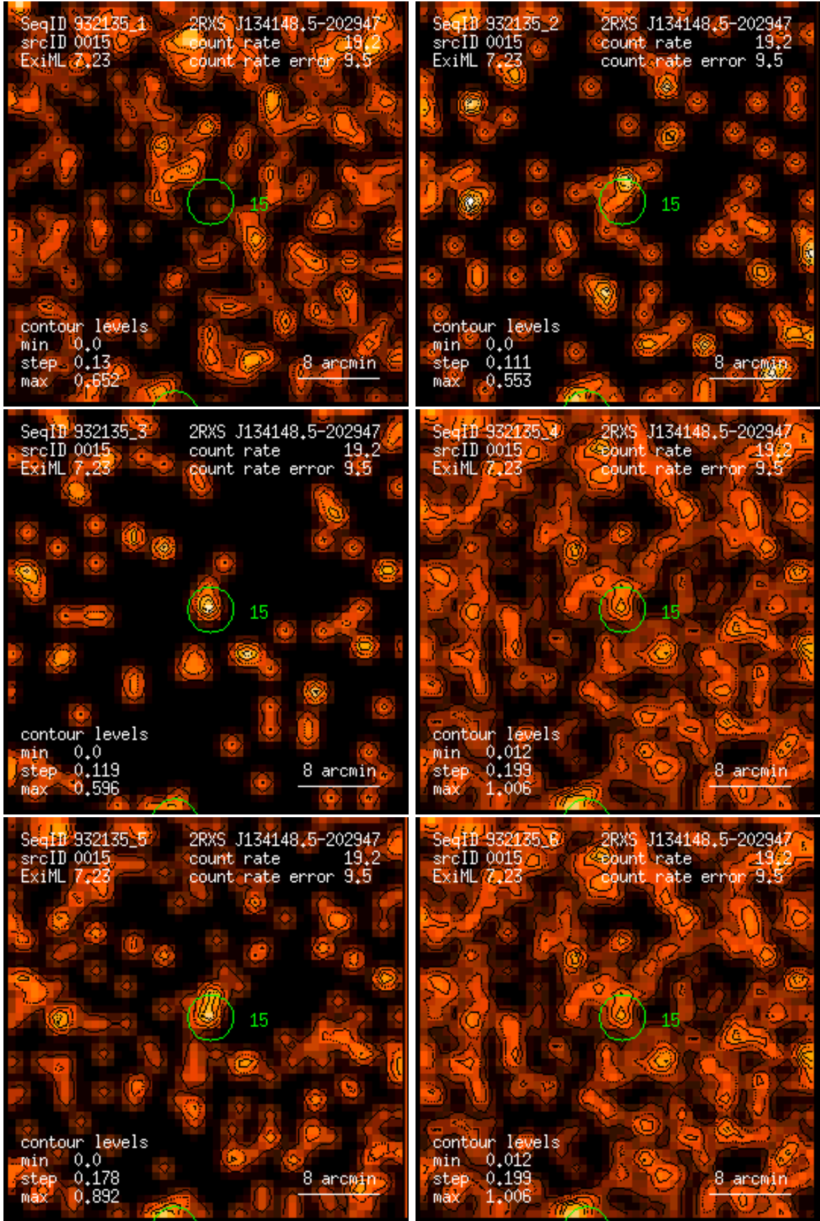
Figure 15: RASS 932135: detection 0015: band rate images, Gaussian filter: (1) PSPC channels 11 – 41, (2) 52 – 90, (3) 91 – 201, (4) 11 – 235, (5) 52 – 201, (6) 11 – 201. Broad band rates in counts/ks. Band rate contour levels in counts/ks/arcmin 2 .
