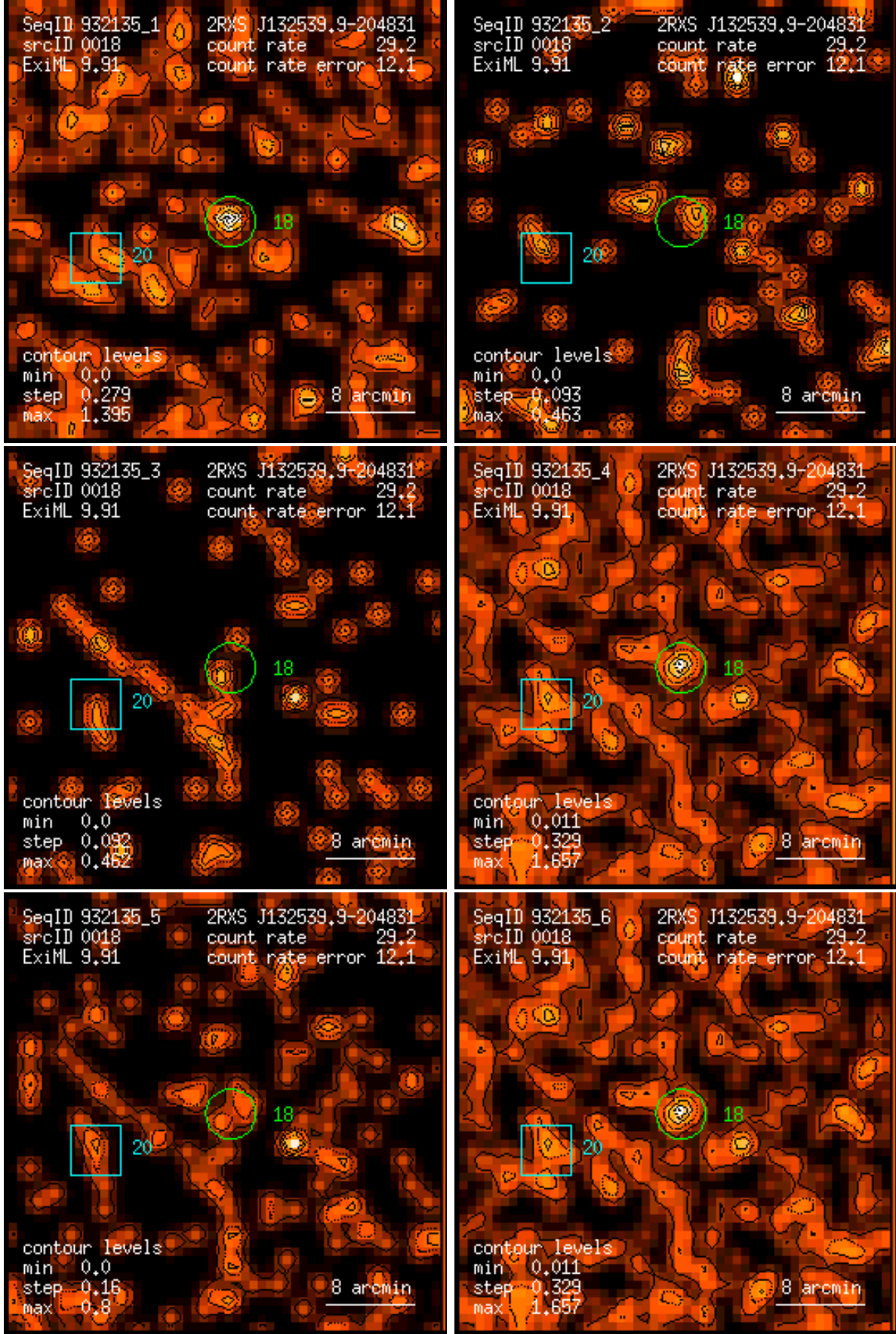
Figure 18: RASS 932135: detection 0018: band rate images, Gaussian filter: (1) PSPC channels 11 – 41, (2) 52 – 90, (3) 91 – 201, (4) 11 – 235, (5) 52 – 201, (6) 11 – 201. Broad band rates in counts/ks. Band rate contour levels in counts/ks/arcmin 2 .
