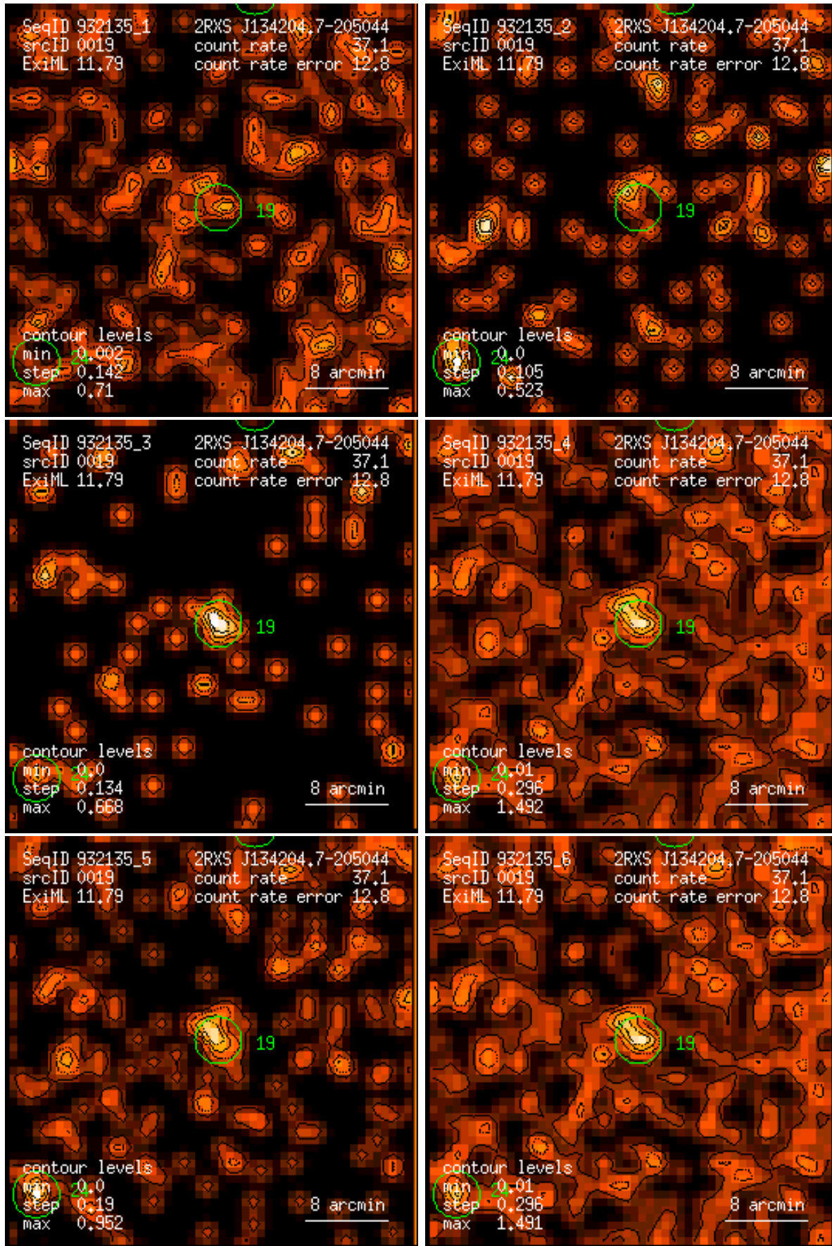
Figure 19: RASS 932135: detection 0019: band rate images, Gaussian filter: (1) PSPC channels 11 – 41, (2) 52 – 90, (3) 91 – 201, (4) 11 – 235, (5) 52 – 201, (6) 11 – 201. Broad band rates in counts/ks. Band rate contour levels in counts/ks/arcmin 2 .
