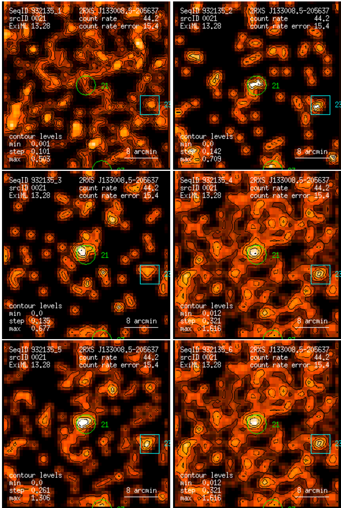
Figure 21: RASS 932135: detection 0021: band rate images, Gaussian filter: (1) PSPC channels 11 – 41, (2) 52 – 90, (3) 91 – 201, (4) 11 – 235, (5) 52 – 201, (6) 11 – 201. Broad band rates in counts/ks. Band rate contour levels in counts/ks/arcmin 2 .
