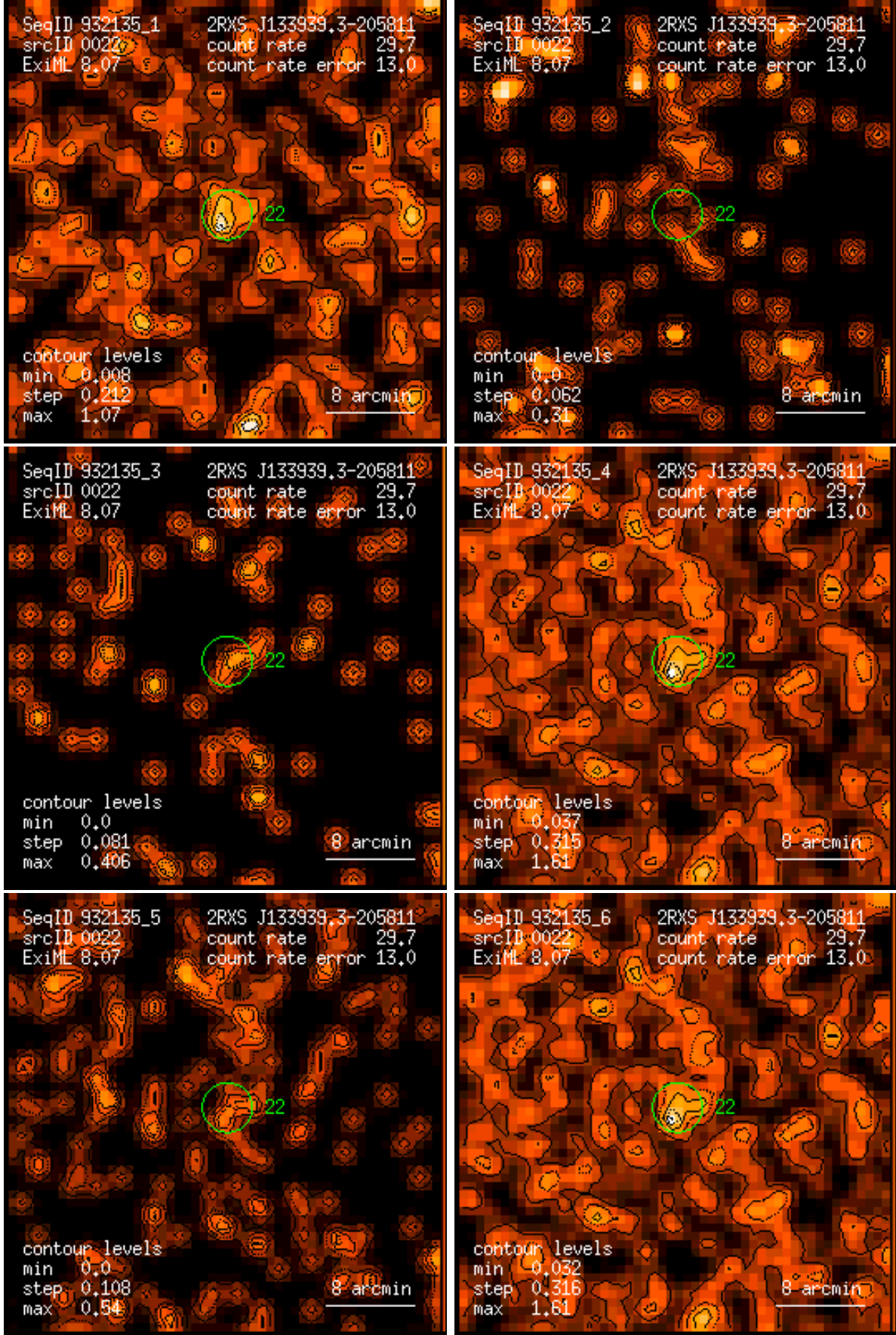
Figure 22: RASS 932135: detection 0022: band rate images, Gaussian filter: (1) PSPC channels 11 – 41, (2) 52 – 90, (3) 91 – 201, (4) 11 – 235, (5) 52 – 201, (6) 11 – 201. Broad band rates in counts/ks. Band rate contour levels in counts/ks/arcmin 2 .
