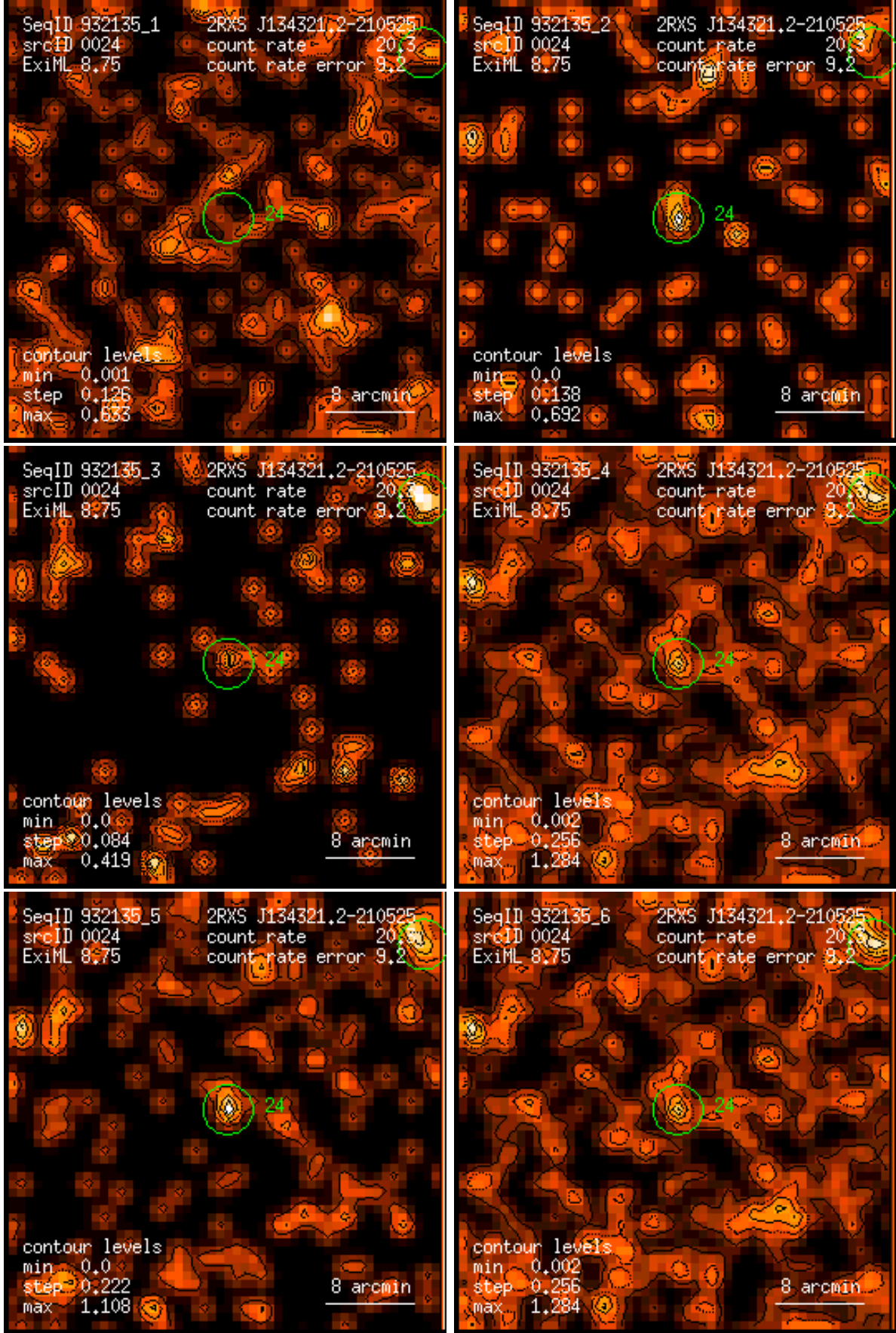
Figure 24: RASS 932135: detection 0024: band rate images, Gaussian filter: (1) PSPC channels 11 – 41, (2) 52 – 90, (3) 91 – 201, (4) 11 – 235, (5) 52 – 201, (6) 11 – 201. Broad band rates in counts/ks. Band rate contour levels in counts/ks/arcmin 2 .
