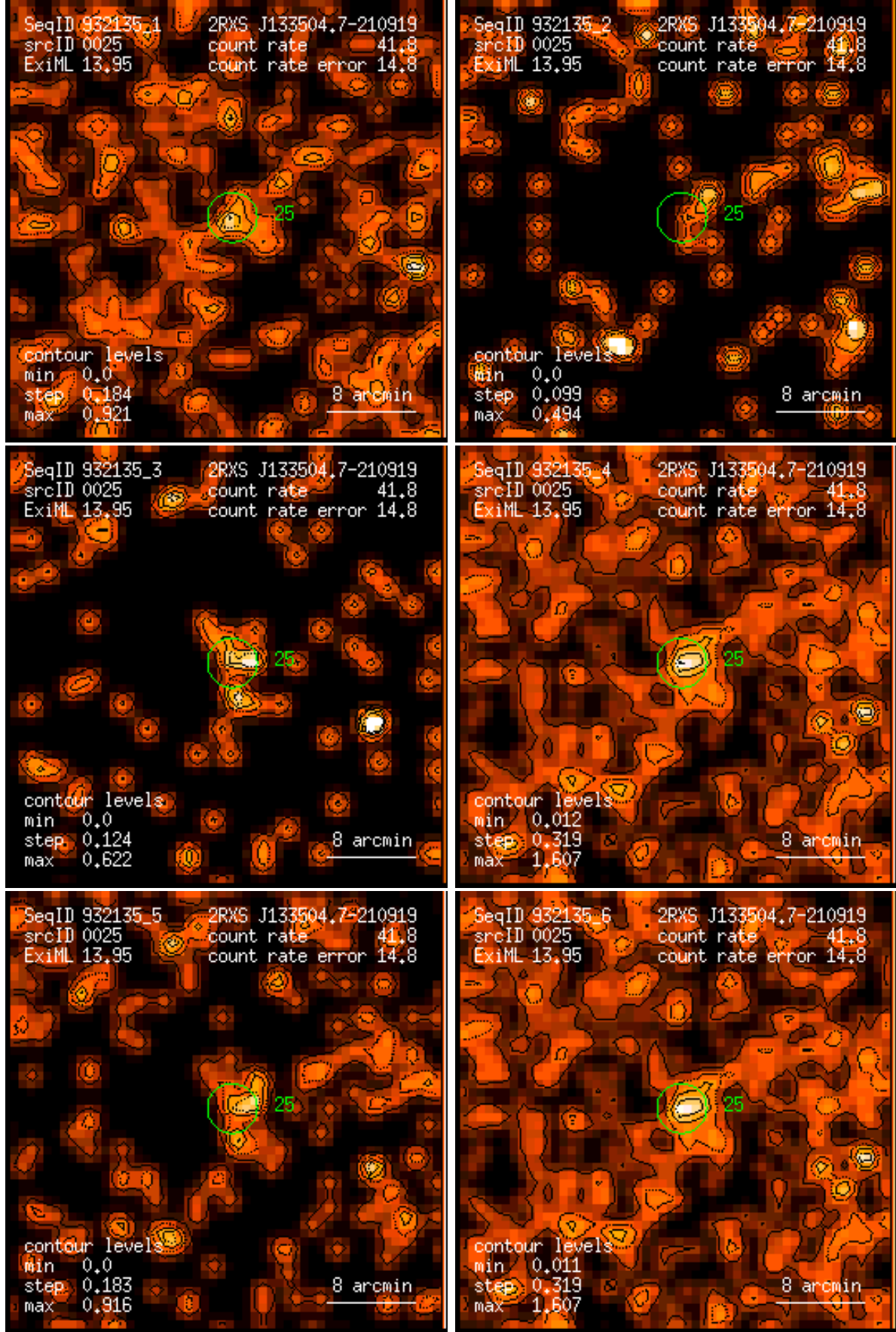
Figure 25: RASS 932135: detection 0025: band rate images, Gaussian filter: (1) PSPC channels 11 – 41, (2) 52 – 90, (3) 91 – 201, (4) 11 – 235, (5) 52 – 201, (6) 11 – 201. Broad band rates in counts/ks. Band rate contour levels in counts/ks/arcmin 2 .
