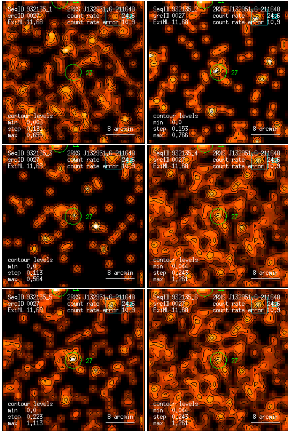
Figure 27: RASS 932135: detection 0027: band rate images, Gaussian filter: (1) PSPC channels 11 – 41, (2) 52 – 90, (3) 91 – 201, (4) 11 – 235, (5) 52 – 201, (6) 11 – 201. Broad band rates in counts/ks. Band rate contour levels in counts/ks/arcmin 2 .
