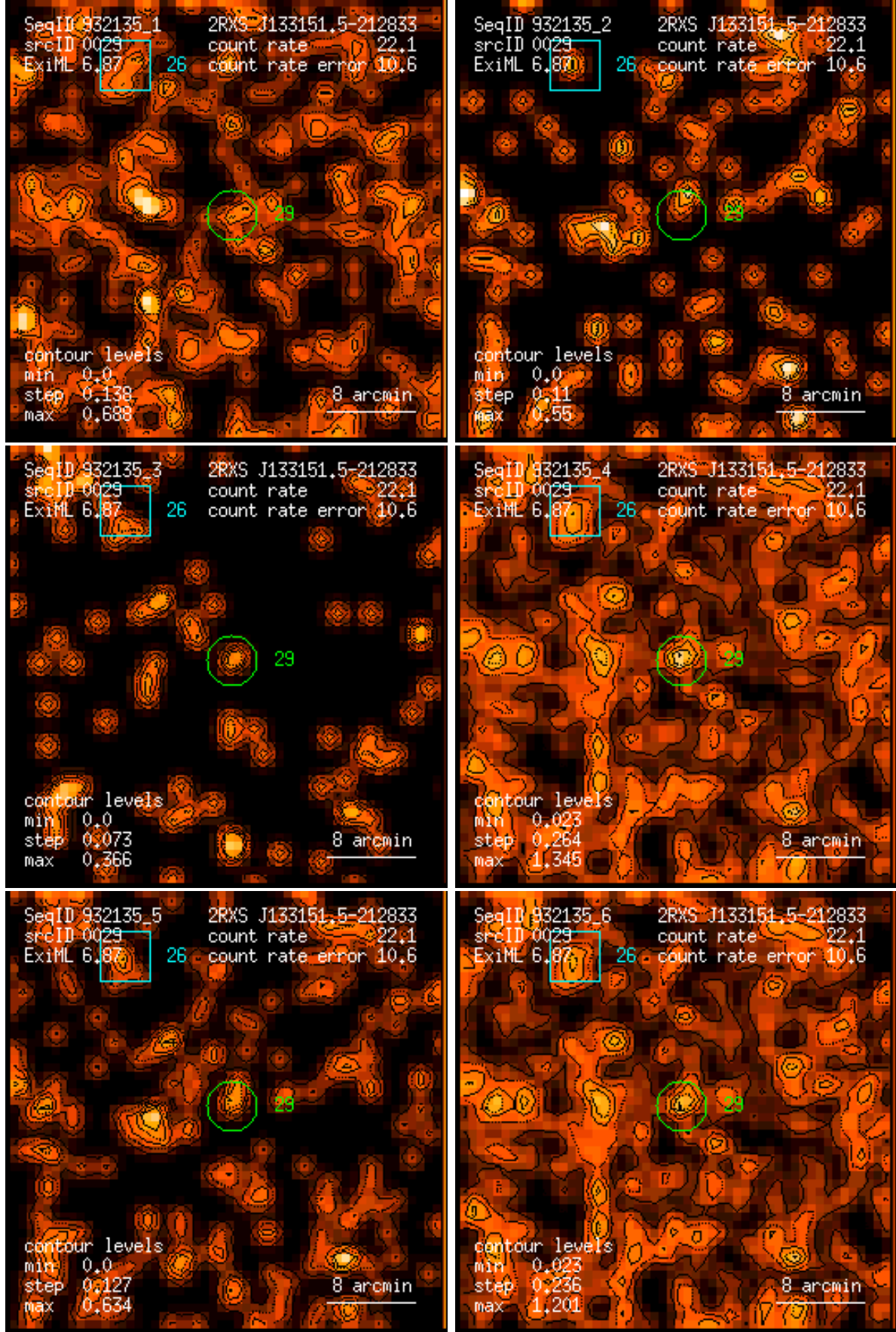
Figure 29: RASS 932135: detection 0029: band rate images, Gaussian filter: (1) PSPC channels 11 – 41, (2) 52 – 90, (3) 91 – 201, (4) 11 – 235, (5) 52 – 201, (6) 11 – 201. Broad band rates in counts/ks. Band rate contour levels in counts/ks/arcmin 2 .
