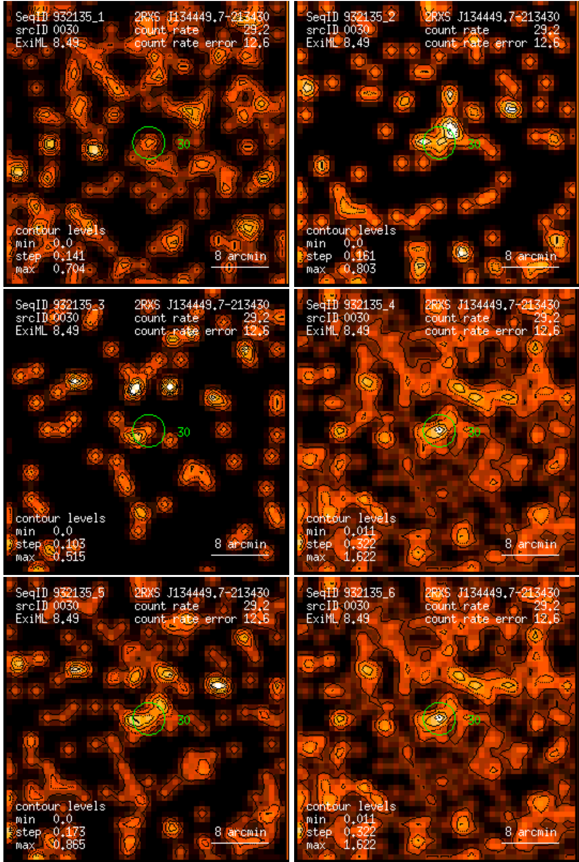
Figure 30: RASS 932135: detection 0030: band rate images, Gaussian filter: (1) PSPC channels 11 – 41, (2) 52 – 90, (3) 91 – 201, (4) 11 – 235, (5) 52 – 201, (6) 11 – 201. Broad band rates in counts/ks. Band rate contour levels in counts/ks/arcmin 2 .
