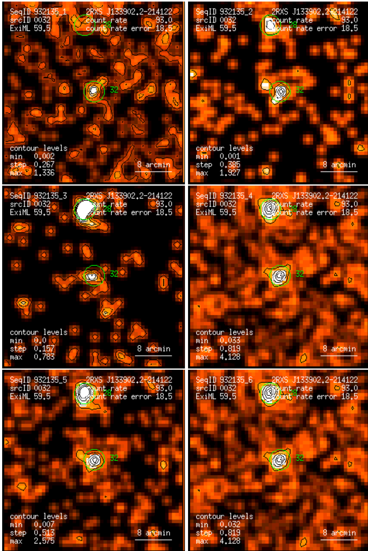
Figure 32: RASS 932135: detection 0032: band rate images, Gaussian filter: (1) PSPC channels 11 – 41, (2) 52 – 90, (3) 91 – 201, (4) 11 – 235, (5) 52 – 201, (6) 11 – 201. Broad band rates in counts/ks. Band rate contour levels in counts/ks/arcmin 2 .
