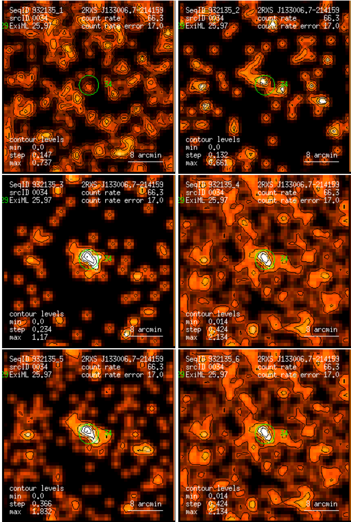
Figure 34: RASS 932135: detection 0034: band rate images, Gaussian filter: (1) PSPC channels 11 – 41, (2) 52 – 90, (3) 91 – 201, (4) 11 – 235, (5) 52 – 201, (6) 11 – 201. Broad band rates in counts/ks. Band rate contour levels in counts/ks/arcmin 2 .
