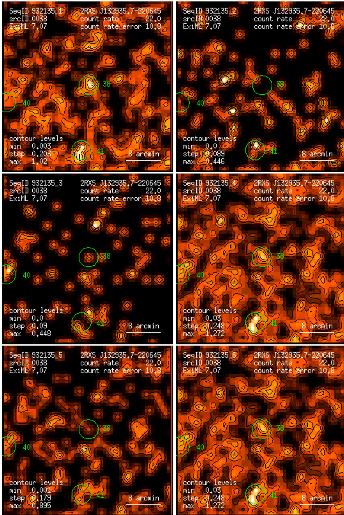
Figure 38: RASS 932135: detection 0038: band rate images, Gaussian filter: (1) PSPC channels 11 – 41, (2) 52 – 90, (3) 91 – 201, (4) 11 – 235, (5) 52 – 201, (6) 11 – 201. Broad band rates in counts/ks. Band rate contour levels in counts/ks/arcmin 2 .
