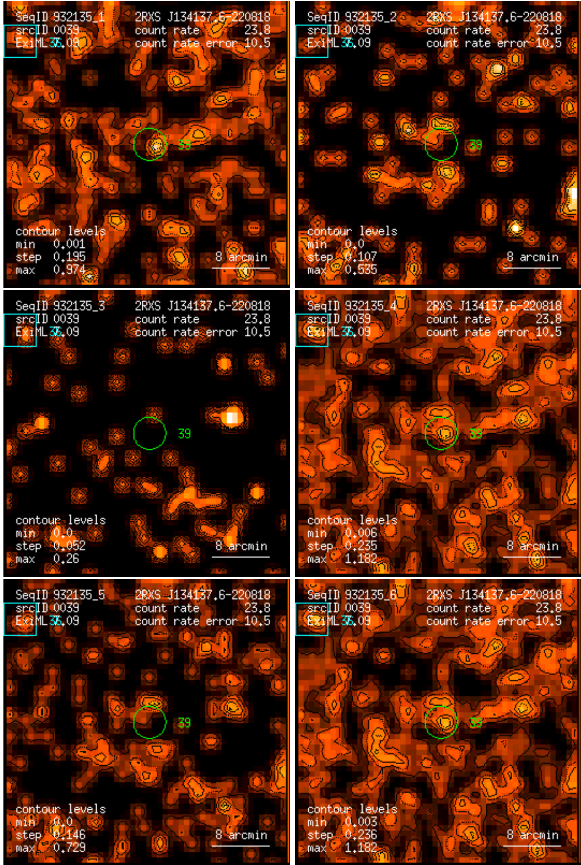
Figure 39: RASS 932135: detection 0039: band rate images, Gaussian filter: (1) PSPC channels 11 – 41, (2) 52 – 90, (3) 91 – 201, (4) 11 – 235, (5) 52 – 201, (6) 11 – 201. Broad band rates in counts/ks. Band rate contour levels in counts/ks/arcmin 2 .
