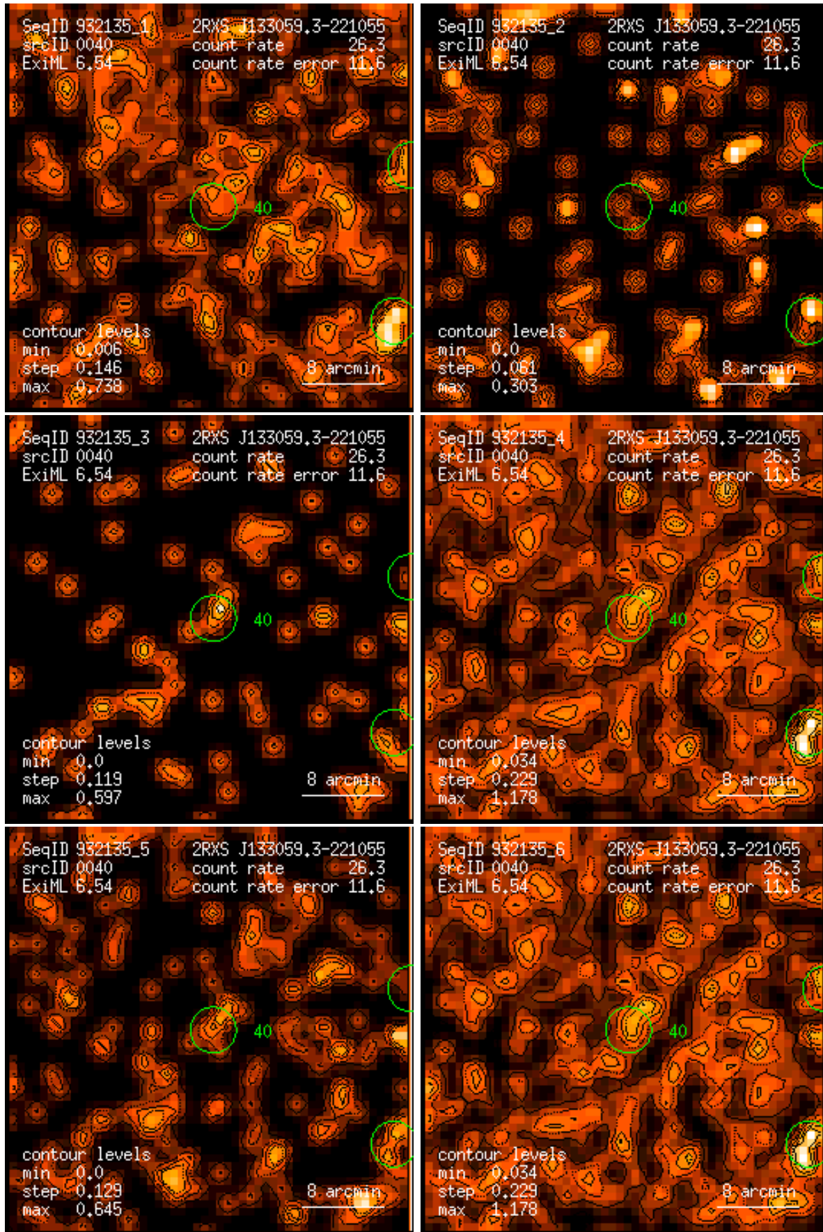
Figure 40: RASS 932135: detection 0040: band rate images, Gaussian filter: (1) PSPC channels 11 – 41, (2) 52 – 90, (3) 91 – 201, (4) 11 – 235, (5) 52 – 201, (6) 11 – 201. Broad band rates in counts/ks. Band rate contour levels in counts/ks/arcmin 2 .
