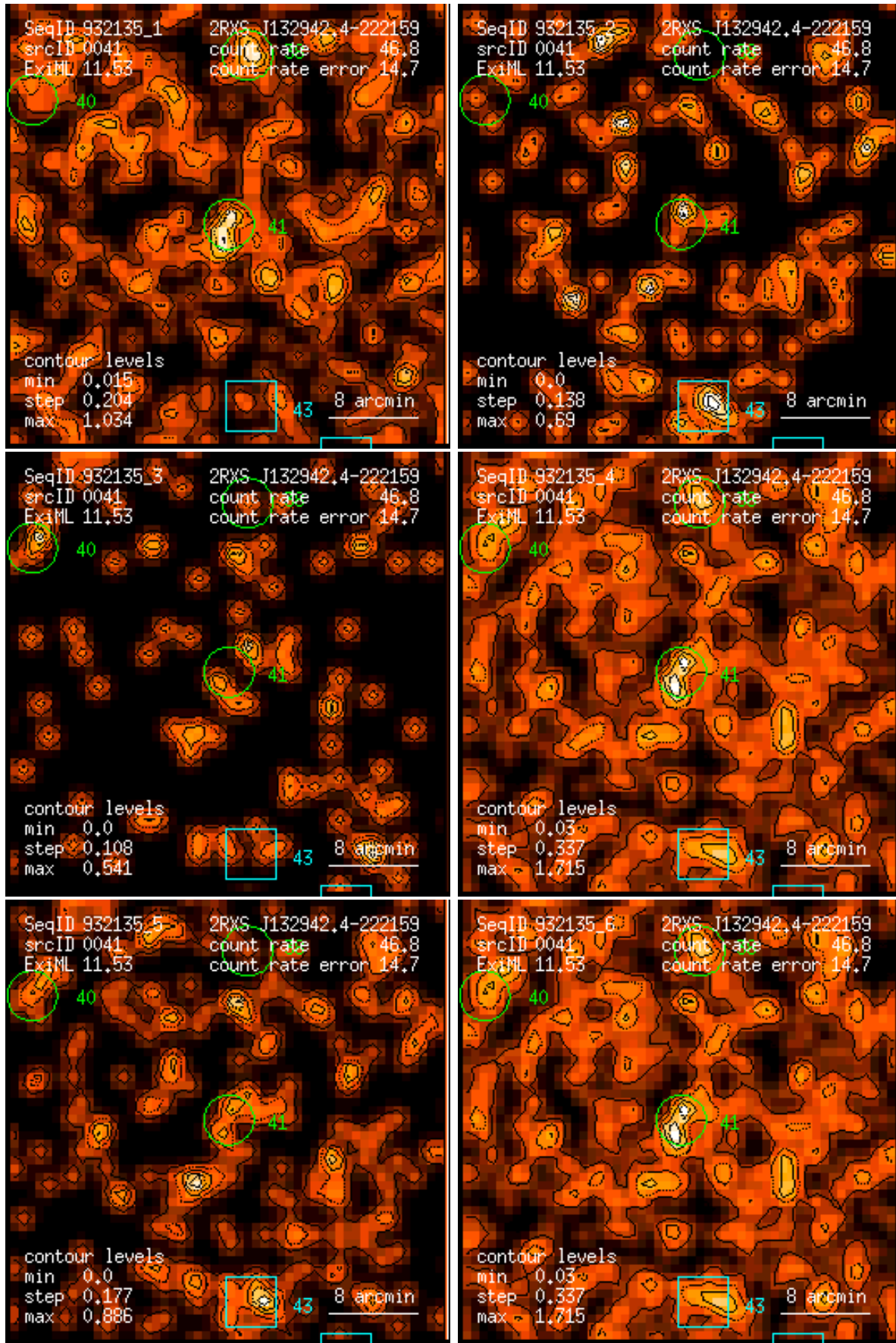
Figure 41: RASS 932135: detection 0041: band rate images, Gaussian filter: (1) PSPC channels 11 – 41, (2) 52 – 90, (3) 91 – 201, (4) 11 – 235, (5) 52 – 201, (6) 11 – 201. Broad band rates in counts/ks. Band rate contour levels in counts/ks/arcmin 2 .
