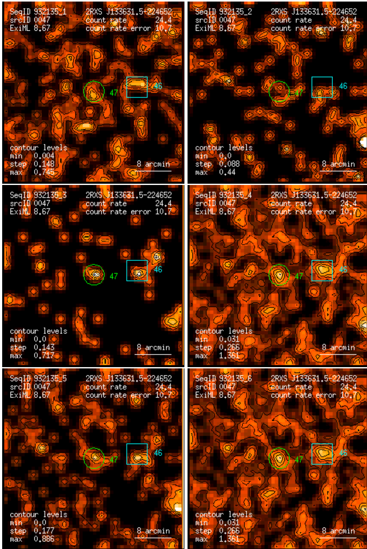
Figure 47: RASS 932135: detection 0047: band rate images, Gaussian filter: (1) PSPC channels 11 – 41, (2) 52 – 90, (3) 91 – 201, (4) 11 – 235, (5) 52 – 201, (6) 11 – 201. Broad band rates in counts/ks. Band rate contour levels in counts/ks/arcmin 2 .
