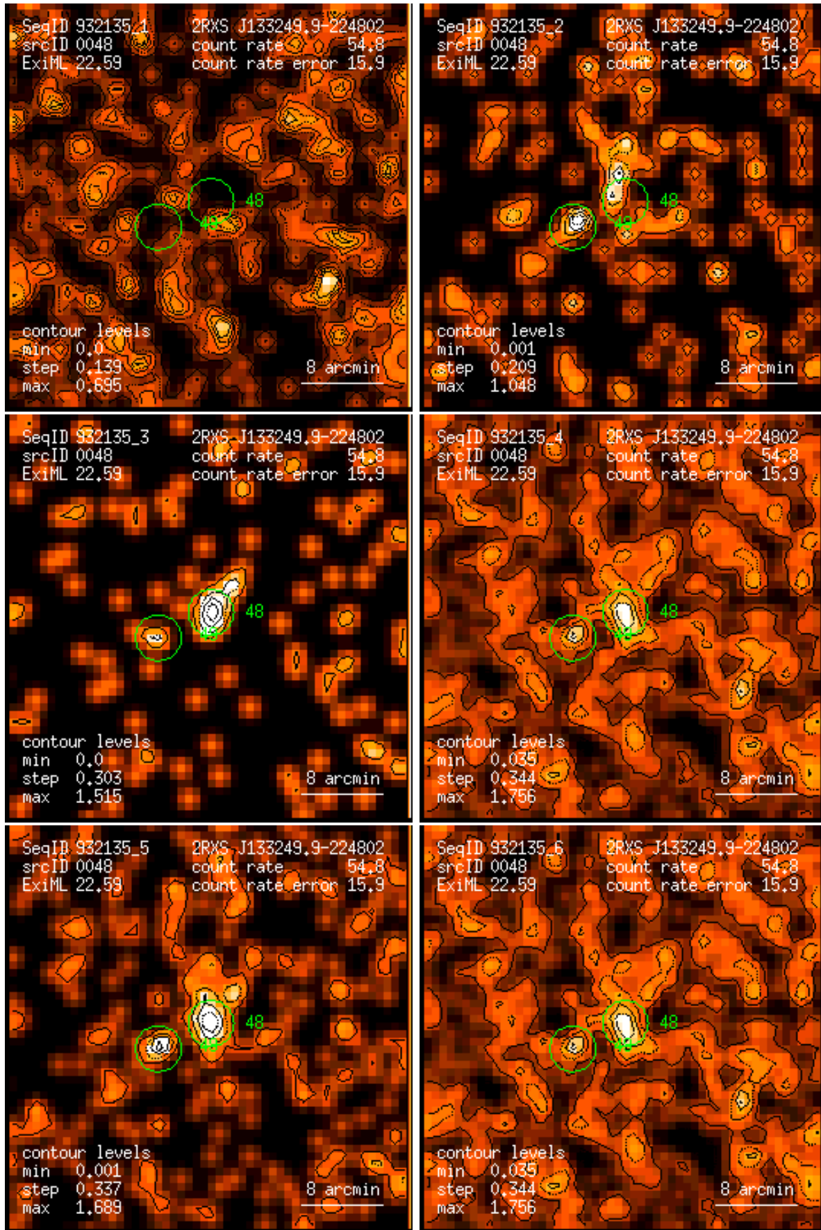
Figure 48: RASS 932135: detection 0048: band rate images, Gaussian filter: (1) PSPC channels 11 – 41, (2) 52 – 90, (3) 91 – 201, (4) 11 – 235, (5) 52 – 201, (6) 11 – 201. Broad band rates in counts/ks. Band rate contour levels in counts/ks/arcmin 2 .
