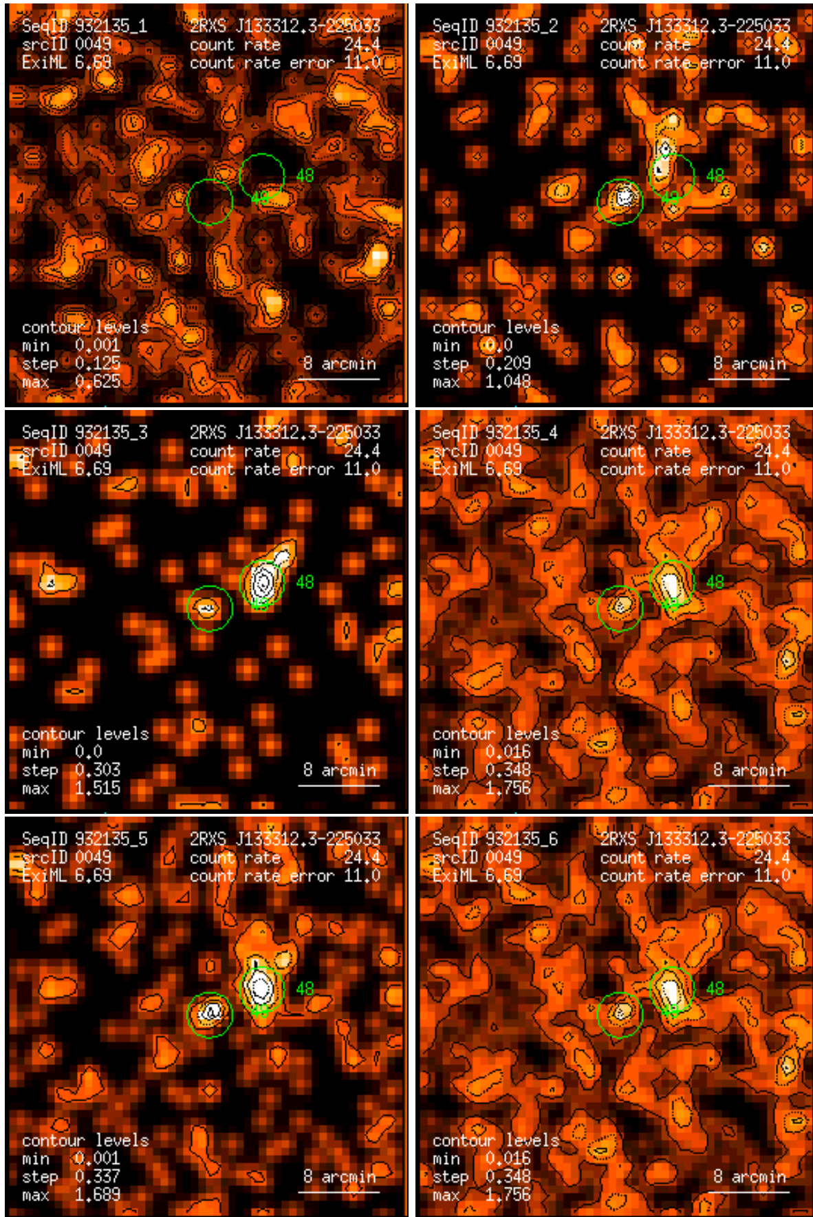
Figure 49: RASS 932135: detection 0049: band rate images, Gaussian filter: (1) PSPC channels 11 – 41, (2) 52 – 90, (3) 91 – 201, (4) 11 – 235, (5) 52 – 201, (6) 11 – 201. Broad band rates in counts/ks. Band rate contour levels in counts/ks/arcmin 2 .
