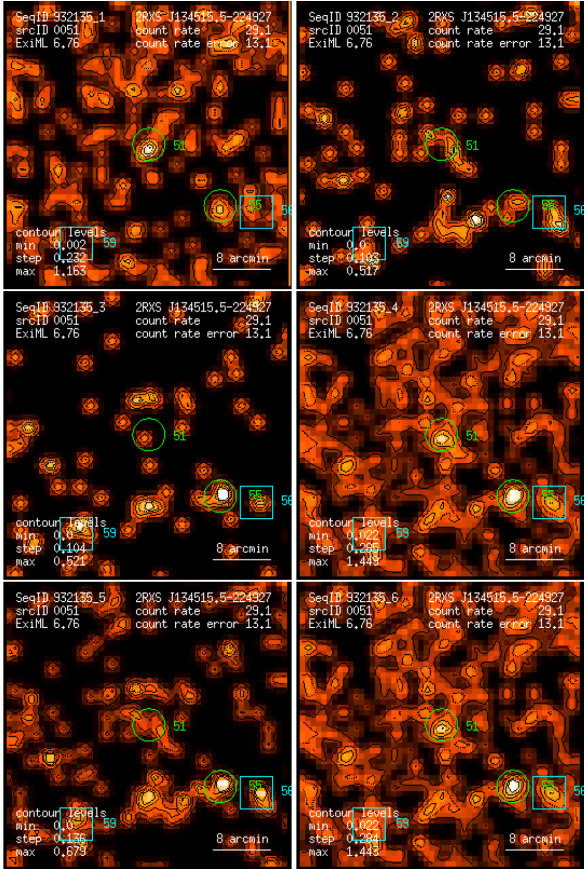
Figure 51: RASS 932135: detection 0051: band rate images, Gaussian filter: (1) PSPC channels 11 – 41, (2) 52 – 90, (3) 91 – 201, (4) 11 – 235, (5) 52 – 201, (6) 11 – 201. Broad band rates in counts/ks. Band rate contour levels in counts/ks/arcmin 2 .
