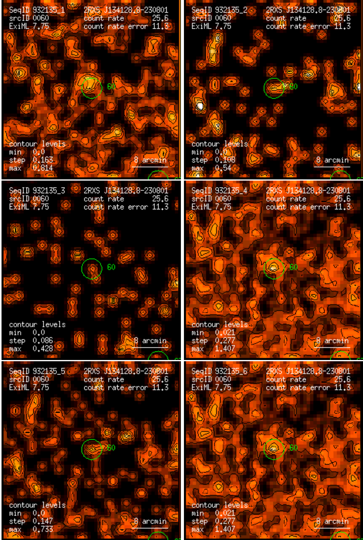
Figure 60: RASS 932135: detection 0060: band rate images, Gaussian filter: (1) PSPC channels 11 – 41, (2) 52 – 90, (3) 91 – 201, (4) 11 – 235, (5) 52 – 201, (6) 11 – 201. Broad band rates in counts/ks. Band rate contour levels in counts/ks/arcmin 2 .
