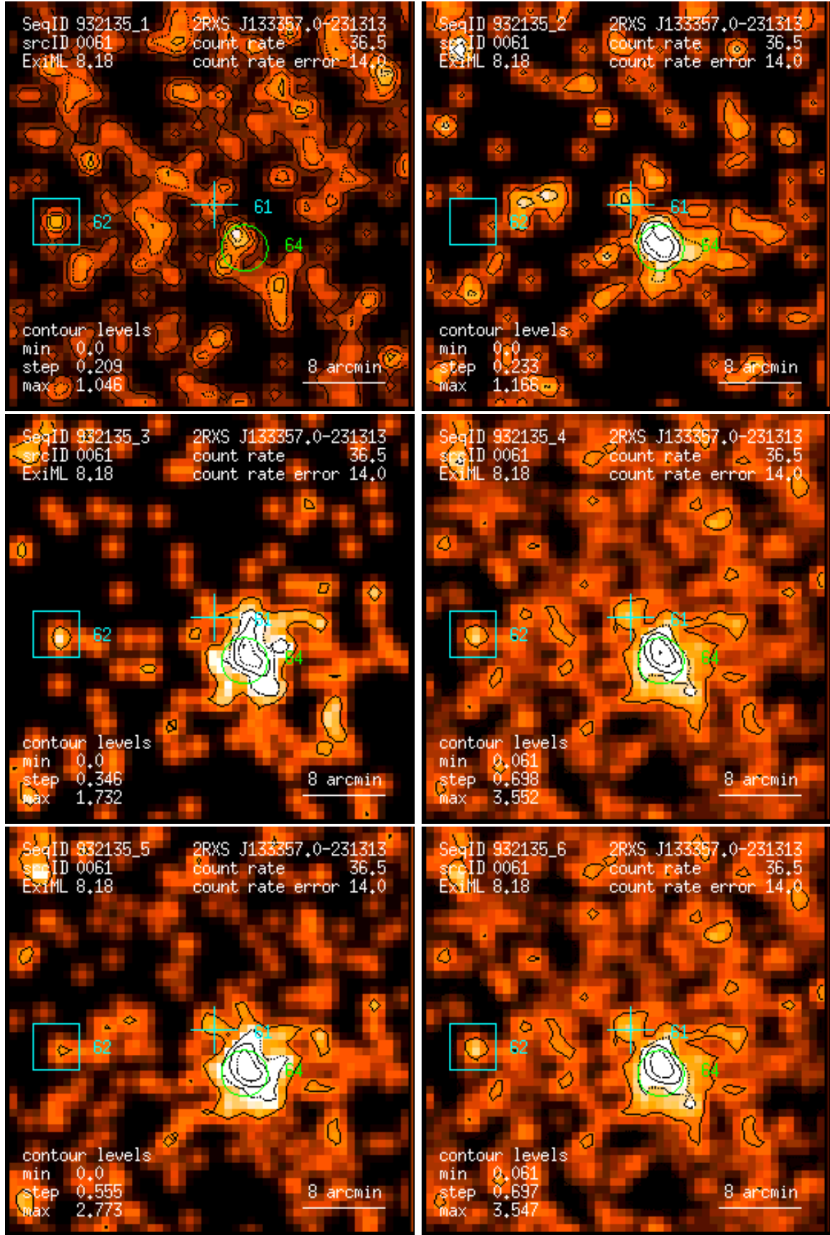
Figure 61: RASS 932135: detection 0061: band rate images, Gaussian filter: (1) PSPC channels 11 – 41, (2) 52 – 90, (3) 91 – 201, (4) 11 – 235, (5) 52 – 201, (6) 11 – 201. Broad band rates in counts/ks. Band rate contour levels in counts/ks/arcmin 2 .
