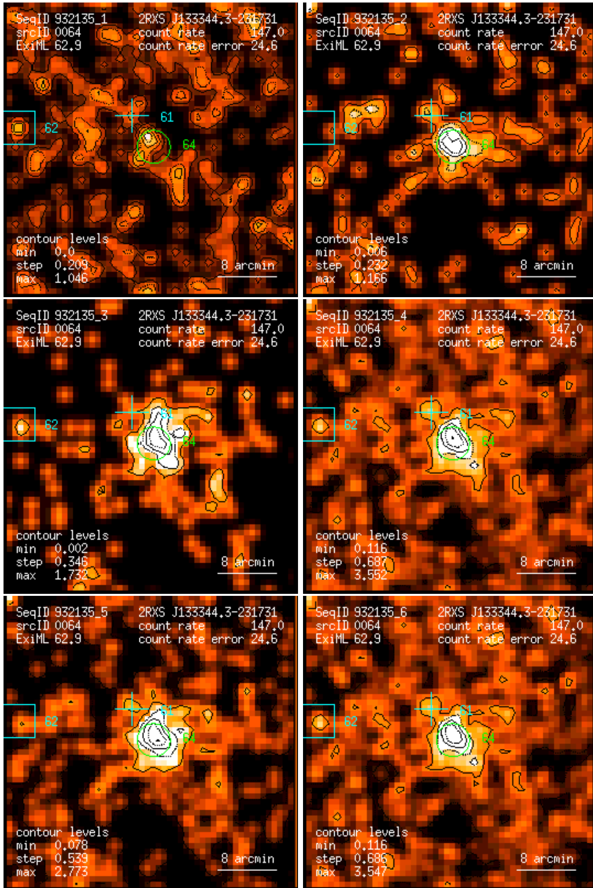
Figure 64: RASS 932135: detection 0064: band rate images, Gaussian filter: (1) PSPC channels 11 – 41, (2) 52 – 90, (3) 91 – 201, (4) 11 – 235, (5) 52 – 201, (6) 11 – 201. Broad band rates in counts/ks. Band rate contour levels in counts/ks/arcmin 2 .
