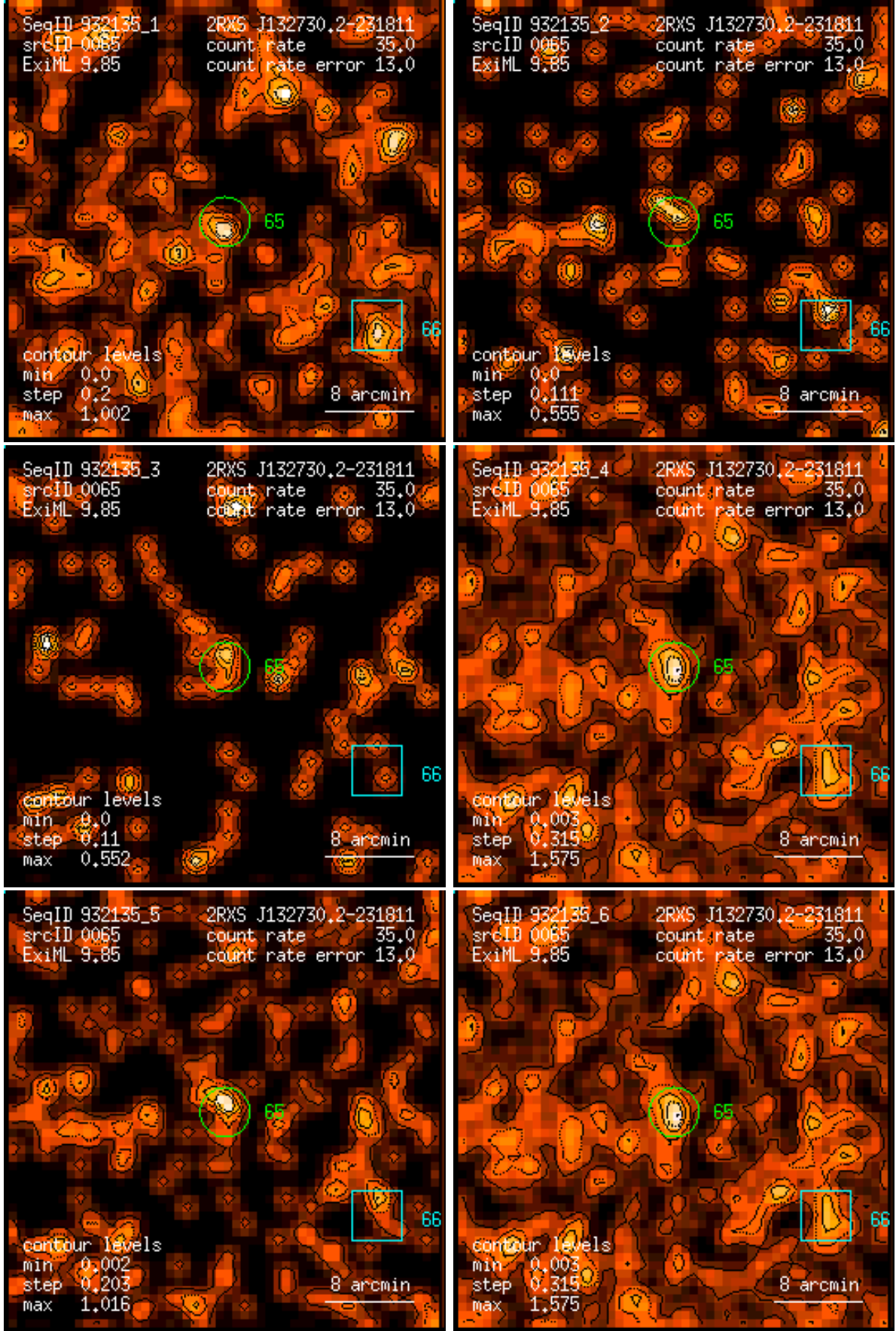
Figure 65: RASS 932135: detection 0065: band rate images, Gaussian filter: (1) PSPC channels 11 – 41, (2) 52 – 90, (3) 91 – 201, (4) 11 – 235, (5) 52 – 201, (6) 11 – 201. Broad band rates in counts/ks. Band rate contour levels in counts/ks/arcmin 2 .
