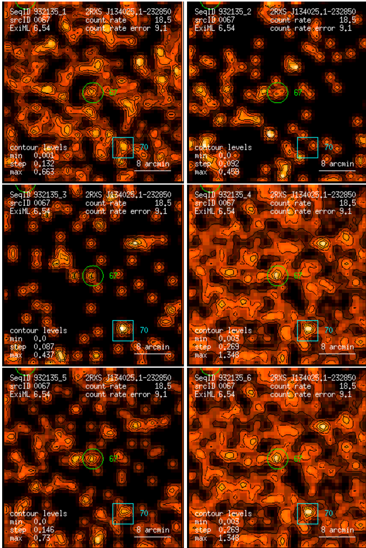
Figure 67: RASS 932135: detection 0067: band rate images, Gaussian filter: (1) PSPC channels 11 – 41, (2) 52 – 90, (3) 91 – 201, (4) 11 – 235, (5) 52 – 201, (6) 11 – 201. Broad band rates in counts/ks. Band rate contour levels in counts/ks/arcmin 2 .
