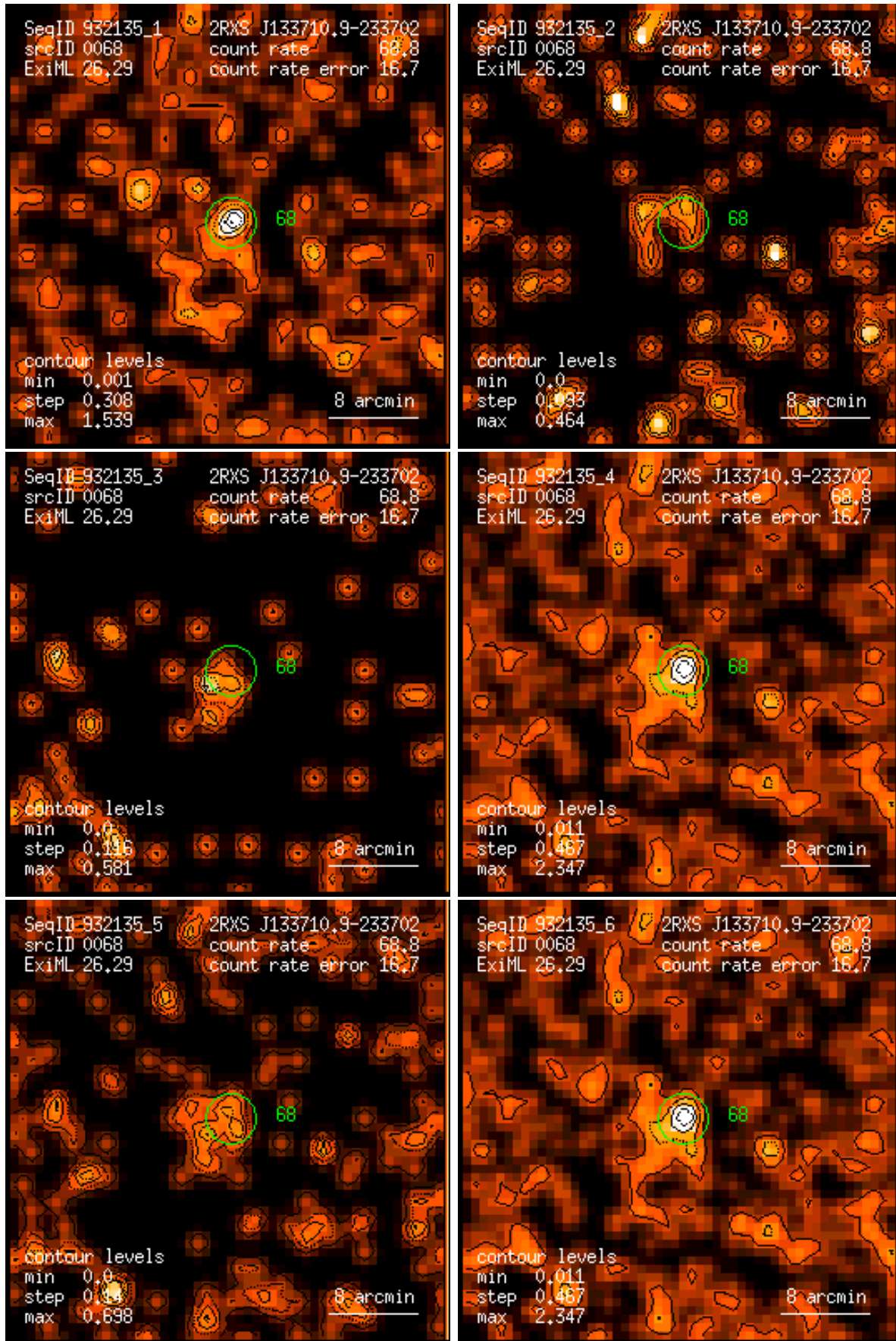
Figure 68: RASS 932135: detection 0068: band rate images, Gaussian filter: (1) PSPC channels 11 – 41, (2) 52 – 90, (3) 91 – 201, (4) 11 – 235, (5) 52 – 201, (6) 11 – 201. Broad band rates in counts/ks. Band rate contour levels in counts/ks/arcmin 2 .
