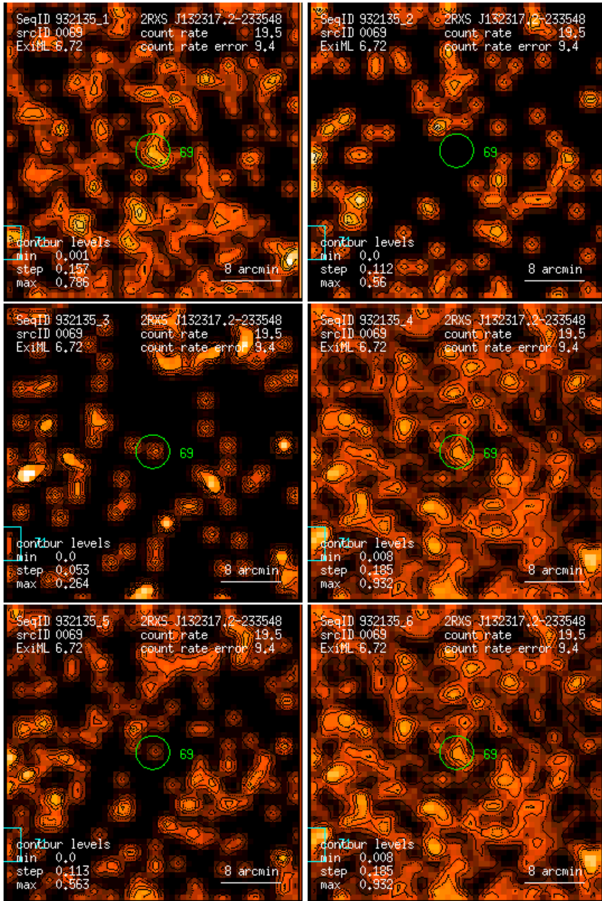
Figure 69: RASS 932135: detection 0069: band rate images, Gaussian filter: (1) PSPC channels 11 – 41, (2) 52 – 90, (3) 91 – 201, (4) 11 – 235, (5) 52 – 201, (6) 11 – 201. Broad band rates in counts/ks. Band rate contour levels in counts/ks/arcmin 2 .
