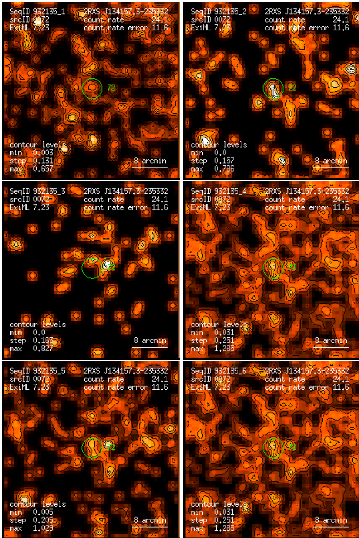
Figure 72: RASS 932135: detection 0072: band rate images, Gaussian filter: (1) PSPC channels 11 – 41, (2) 52 – 90, (3) 91 – 201, (4) 11 – 235, (5) 52 – 201, (6) 11 – 201. Broad band rates in counts/ks. Band rate contour levels in counts/ks/arcmin 2 .
