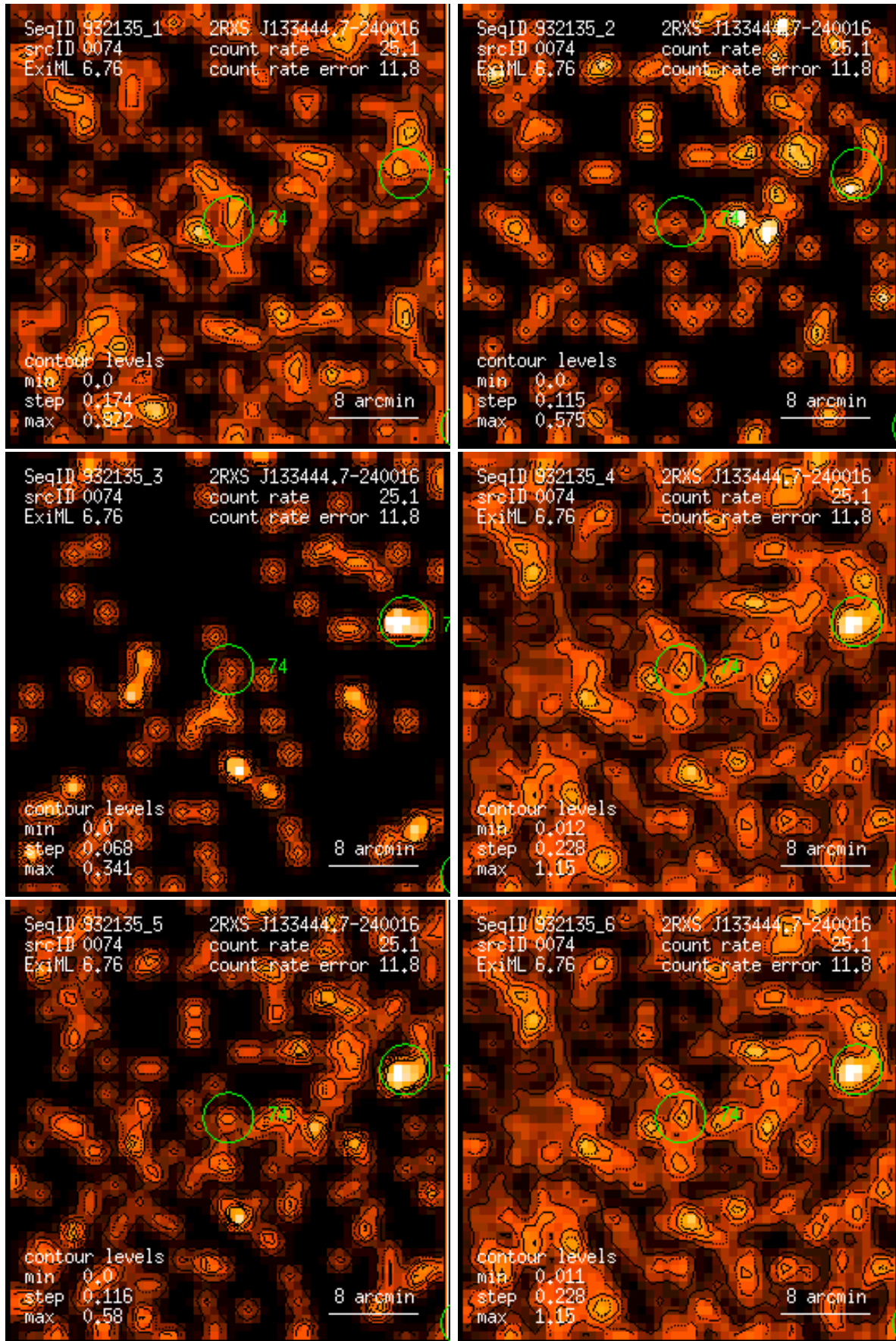
Figure 74: RASS 932135: detection 0074: band rate images, Gaussian filter: (1) PSPC channels 11 – 41, (2) 52 – 90, (3) 91 – 201, (4) 11 – 235, (5) 52 – 201, (6) 11 – 201. Broad band rates in counts/ks. Band rate contour levels in counts/ks/arcmin 2 .
