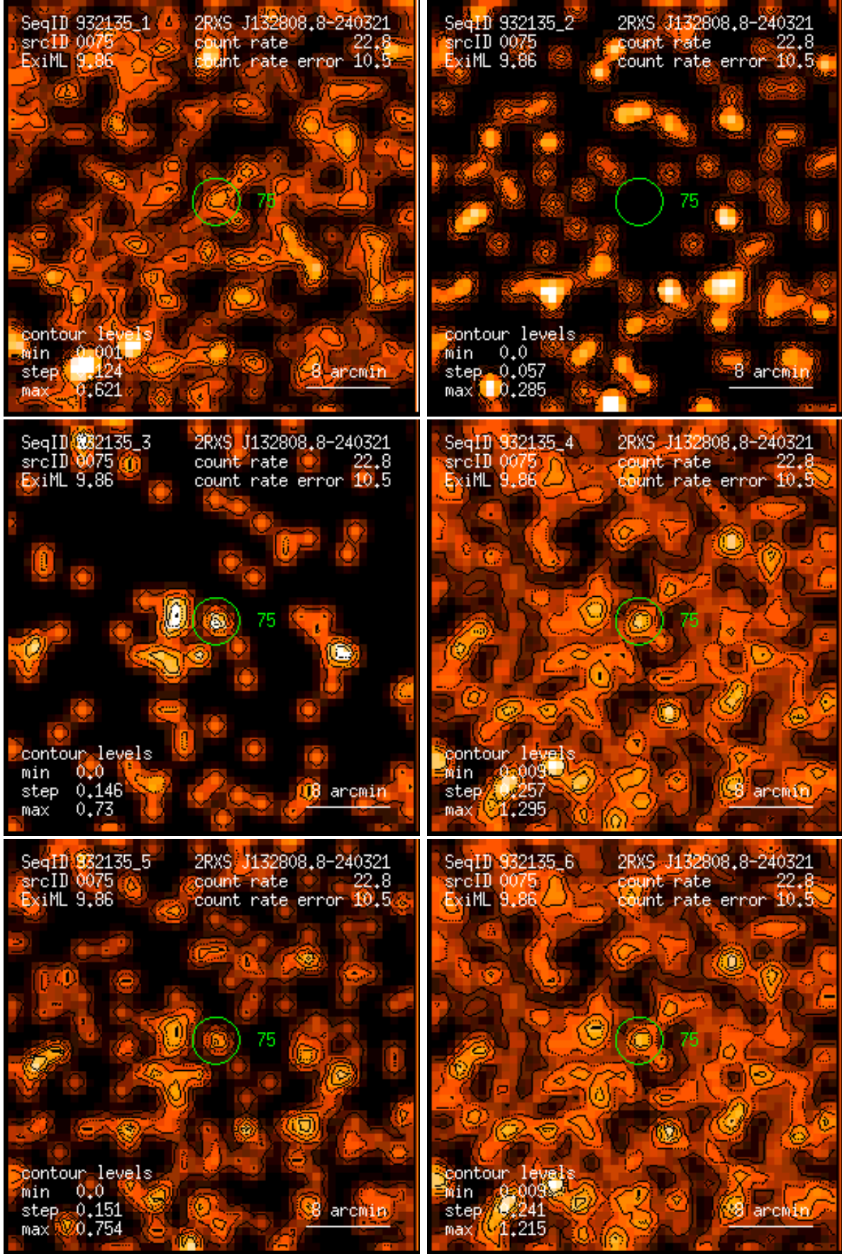
Figure 75: RASS 932135: detection 0075: band rate images, Gaussian filter: (1) PSPC channels 11 – 41, (2) 52 – 90, (3) 91 – 201, (4) 11 – 235, (5) 52 – 201, (6) 11 – 201. Broad band rates in counts/ks. Band rate contour levels in counts/ks/arcmin 2 .
