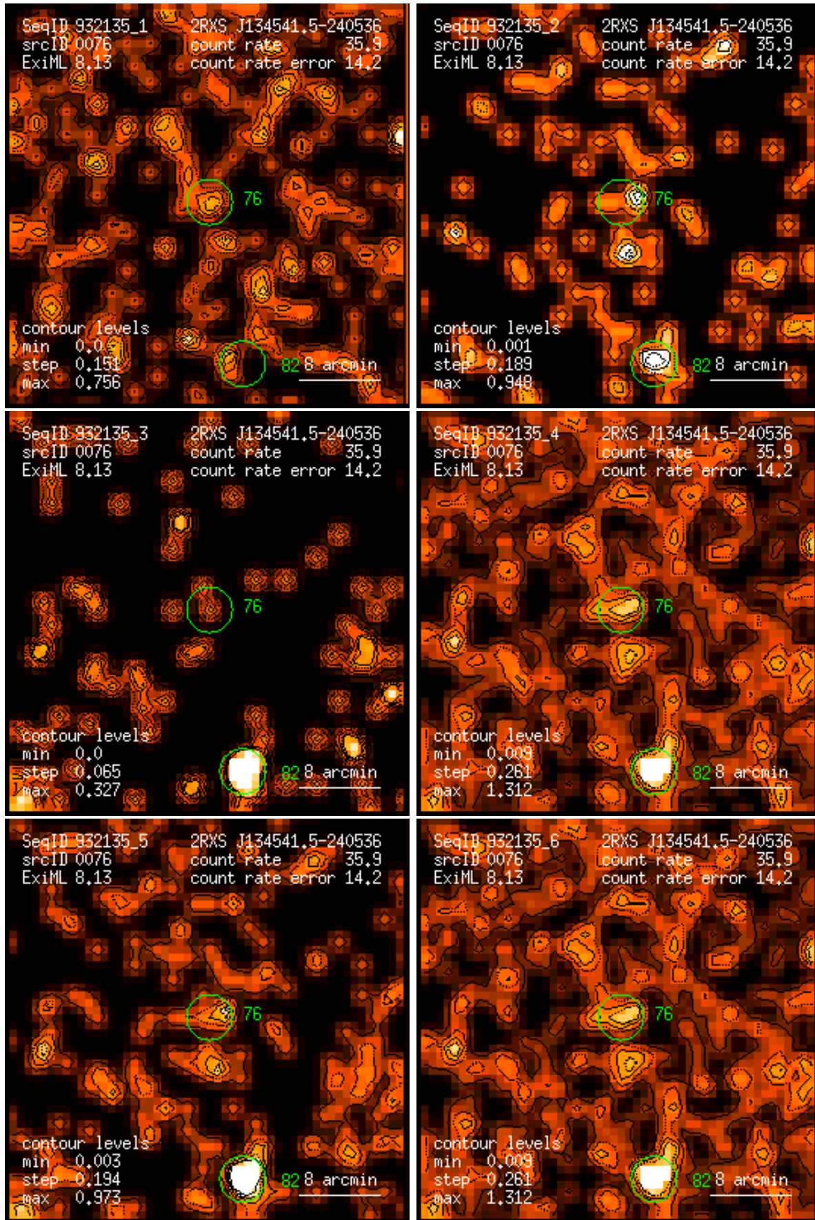
Figure 76: RASS 932135: detection 0076: band rate images, Gaussian filter: (1) PSPC channels 11 – 41, (2) 52 – 90, (3) 91 – 201, (4) 11 – 235, (5) 52 – 201, (6) 11 – 201. Broad band rates in counts/ks. Band rate contour levels in counts/ks/arcmin 2 .
