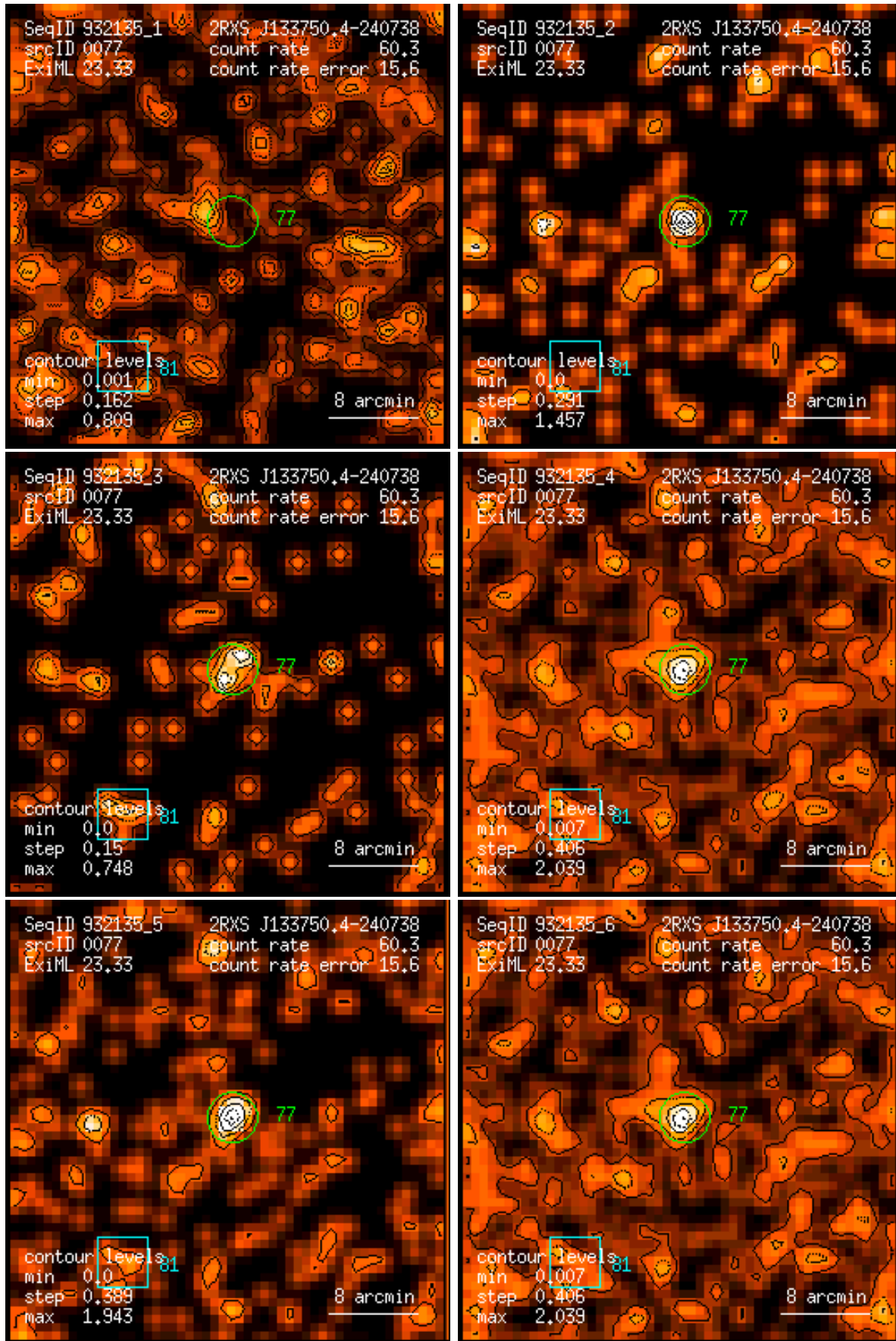
Figure 77: RASS 932135: detection 0077: band rate images, Gaussian filter: (1) PSPC channels 11 – 41, (2) 52 – 90, (3) 91 – 201, (4) 11 – 235, (5) 52 – 201, (6) 11 – 201. Broad band rates in counts/ks. Band rate contour levels in counts/ks/arcmin 2 .
