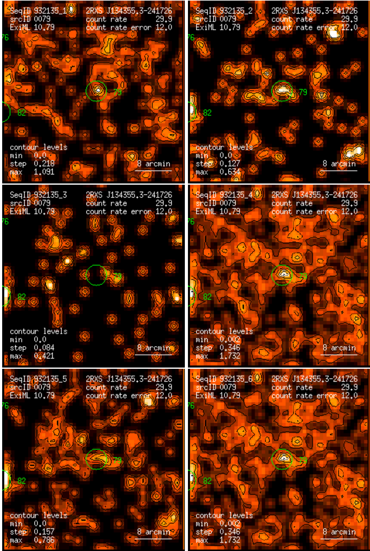
Figure 79: RASS 932135: detection 0079: band rate images, Gaussian filter: (1) PSPC channels 11 – 41, (2) 52 – 90, (3) 91 – 201, (4) 11 – 235, (5) 52 – 201, (6) 11 – 201. Broad band rates in counts/ks. Band rate contour levels in counts/ks/arcmin 2 .
