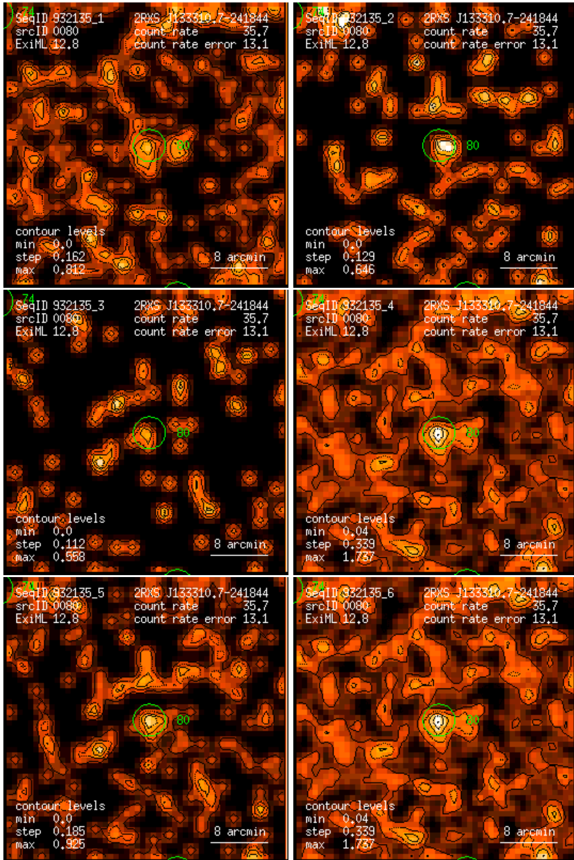
Figure 80: RASS 932135: detection 0080: band rate images, Gaussian filter: (1) PSPC channels 11 – 41, (2) 52 – 90, (3) 91 – 201, (4) 11 – 235, (5) 52 – 201, (6) 11 – 201. Broad band rates in counts/ks. Band rate contour levels in counts/ks/arcmin 2 .
